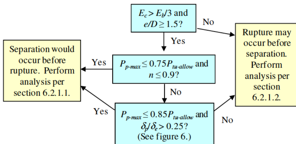
Figure 5—Determining Whether a Joint Separates Before Rupture When Loaded Solely in Tension
