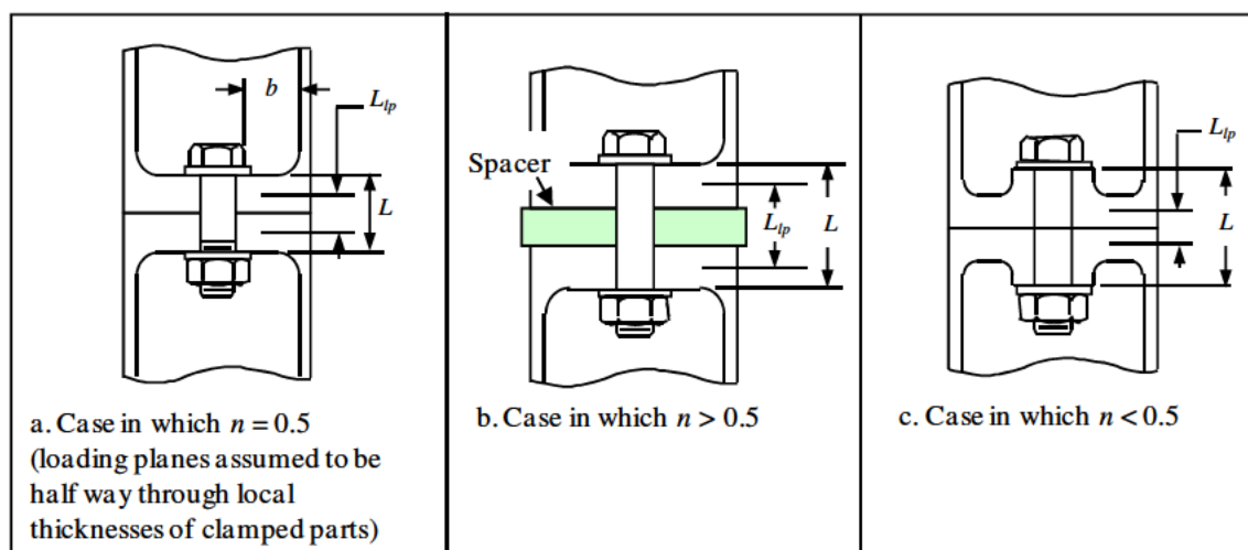
Figure 4—Dimensions Used to Calculate Load-Introduction Factor
