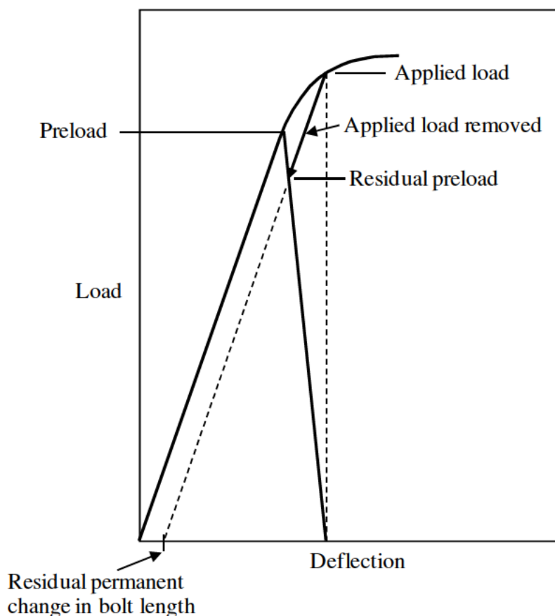
Figure 16—Loss of Preload Resulting from Fastener Yielding
