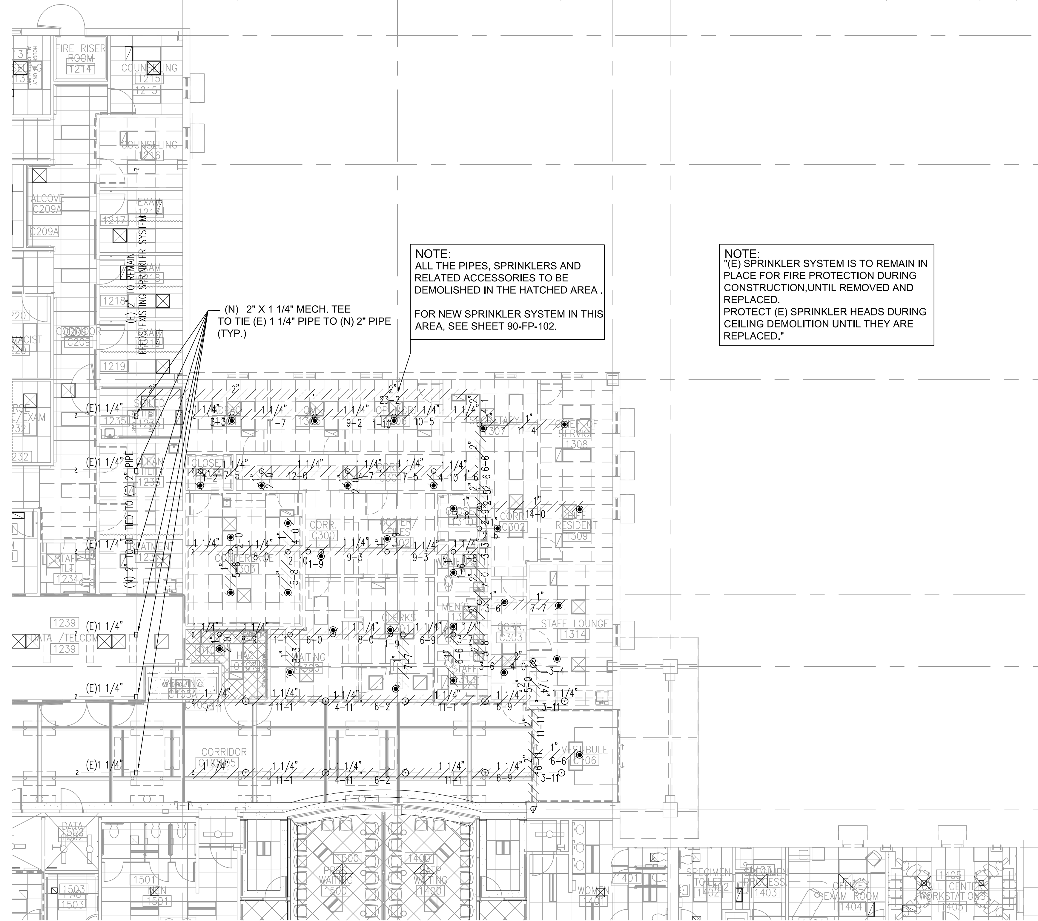
1 FIRE PROTECTION PIPING DEMO PLAN 1/8" = 1'-0"
