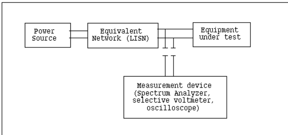
FIGURE 3.4.1.1.1-2 MODEL FOR MEASUREMENT OF INTERFERENCE IN 28V SUPPLY CIRCUITS
