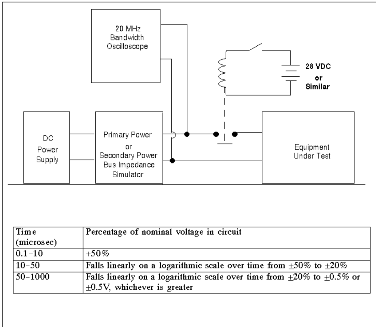
FIGURE 3.4.3.1.2-1 CONDUCTED EMISSIONS (SPIKE) TEST SETUP FOR EQUIPMENT USING USOS PRIMARY OR SECONDARY POWER
