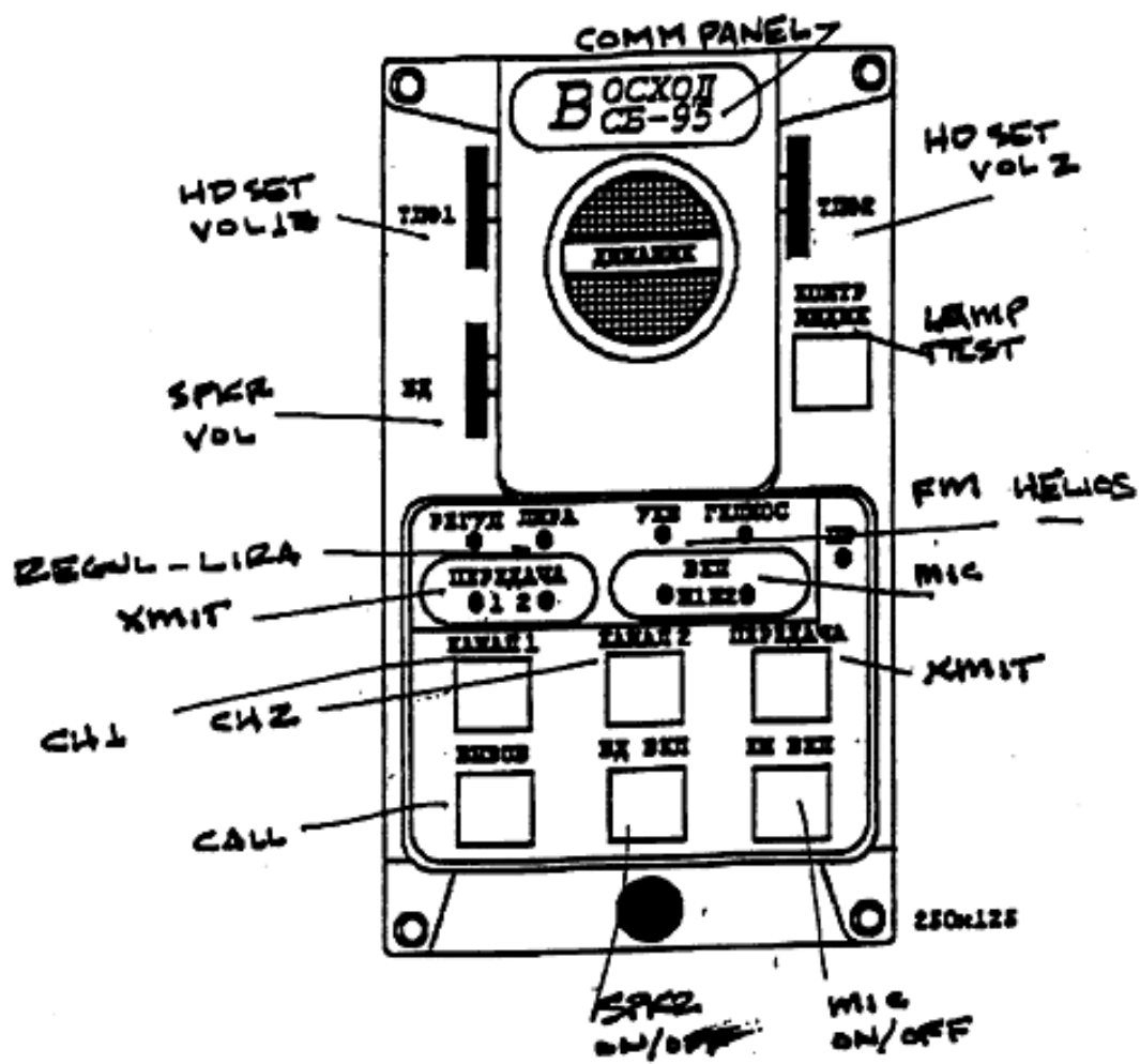
FIGURE 6.4.7.1.4.8-3 COMMUNICATION PANEL
