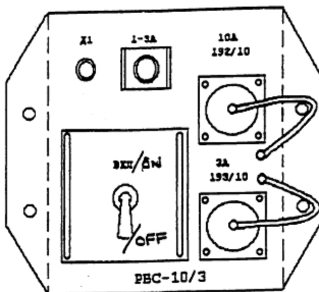
FIGURE 6.4.7.1.4.8-2 ON BOARD RECEPTACLE RBS -10/3
