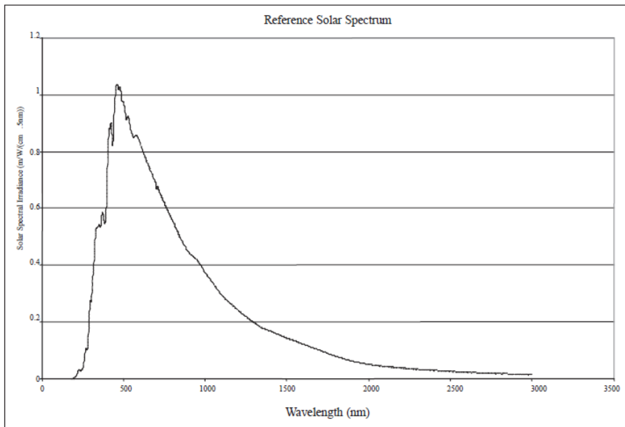
FIGURE 7.1.4.8.4-1 SOLAR SPECTRUM
