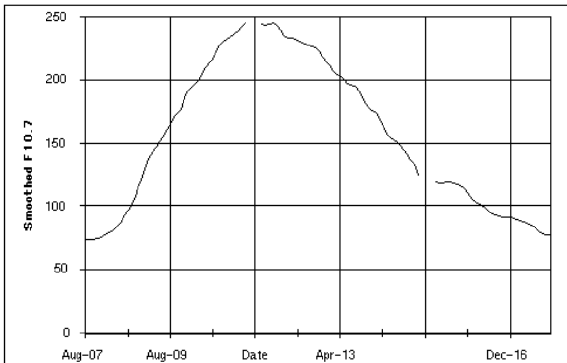
FIGURE 3.2.1.2-3 NASA DESIGN PROFILES FOR SOLAR CYCLE 24; F10.7 ASSUMING A MOST LIKELY START DATE OF AUGUST 2007
