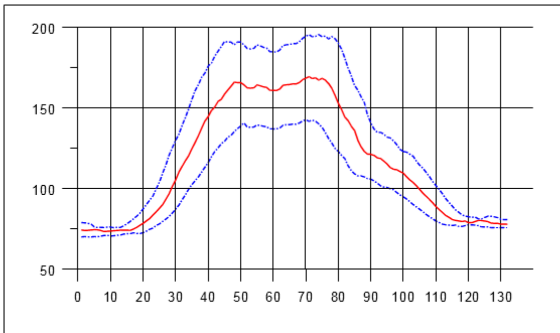
FIGURE 3.2.1.1-1 RSA FEB-96 DESIGN ATMOSPHERE PROFILE FOR SOLAR CYCLE 23: 13 MONTH SMOOTHED F_{10.7}
