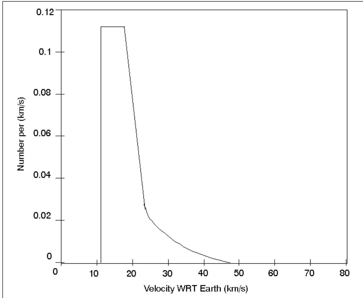
FIGURE 3.8.1-1 NORMALIZED METEOROID VELOCITY DISTRIBUTION FROM EQUATION 3.8.1,1
