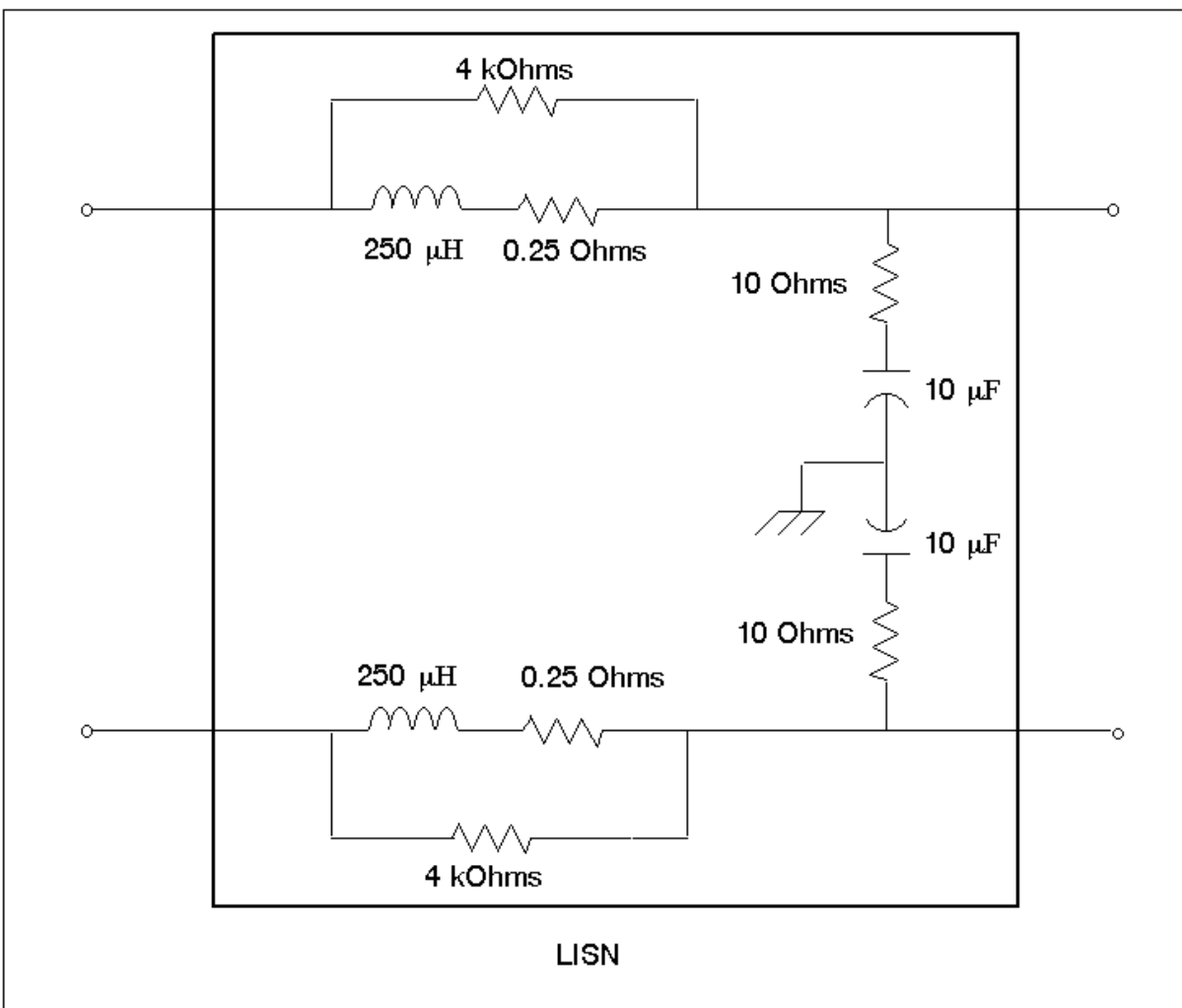
FIGURE 3.4.3.1.1-4 USOS PRIMARY POWER BUS EQUIVALENT NETWORK
