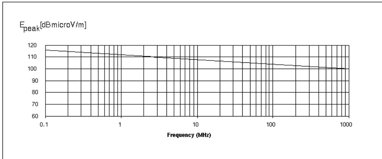
FIGURE 3.4.1.2.4-2 EQUIPMENT IMMUNITY REQUIREMENTS (INTENSITY OF THE ELECTRICAL FIELD INSIDE A MODULE)
