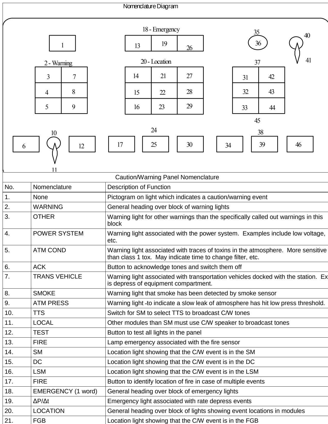
FIGURE 6.4.7.1.4.8-1 CAUTION/WARNING PANEL
