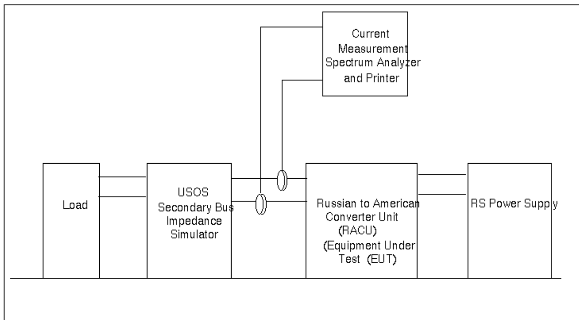
FIGURE 3.4.2.1.1-2 CONDUCTED EMISSIONS TEST SETUP FOR EQUIPMENT PROVIDING 120 V SECONDARY POWER
