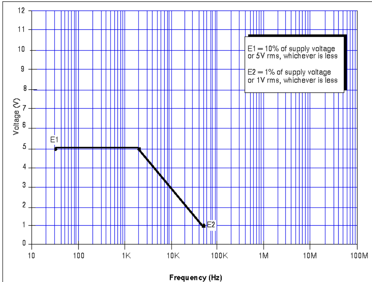
FIGURE 3.4.3.2.1-1 LIMITS OF CONDUCTED INTERFERENCE SUSCEPTIBILITY FOR EQUIPMENT USING THE USOS PRIMARY POWER SUPPLY OR 120 V SECONDARY POWER SUPPLY
