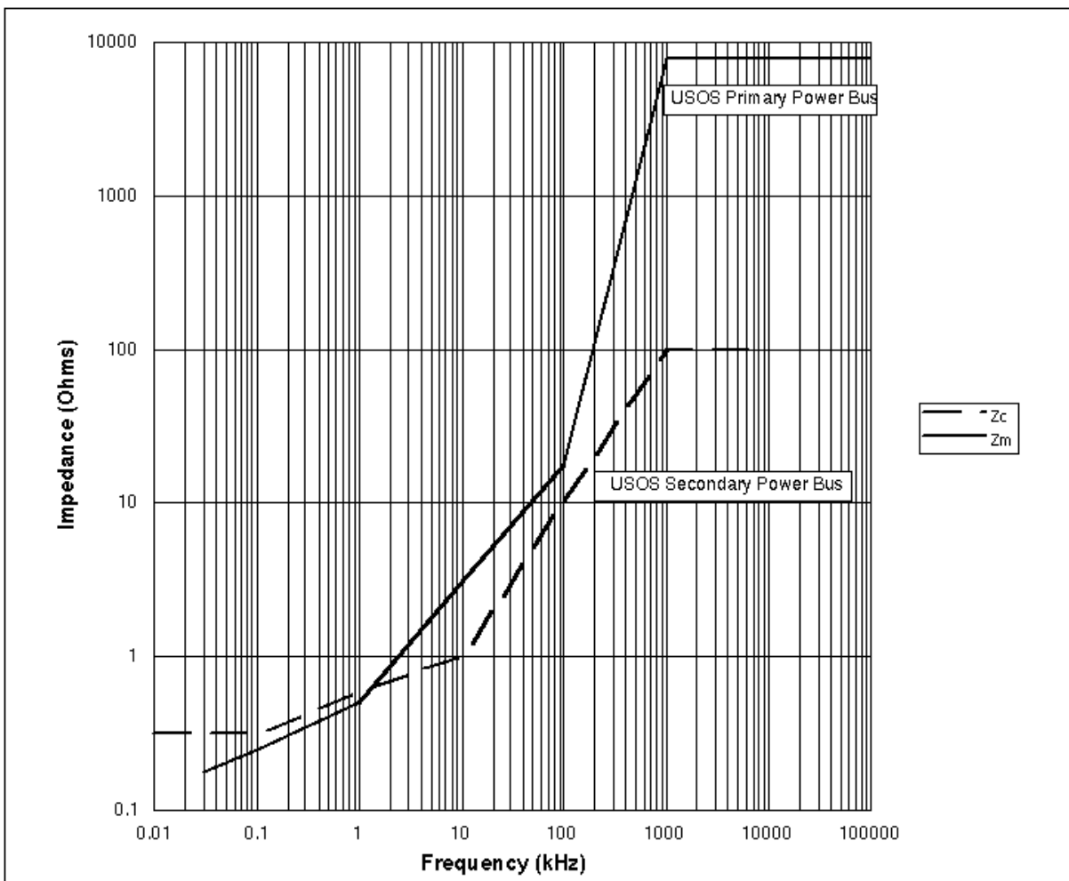
FIGURE 3.4.3.1.1-3 PRIMARY POWER BUS SOURCE IMPEDANCE ( Z_m ) AND SECONDARY POWER BUS SOURCE IMPEDANCE ( Z_c )
