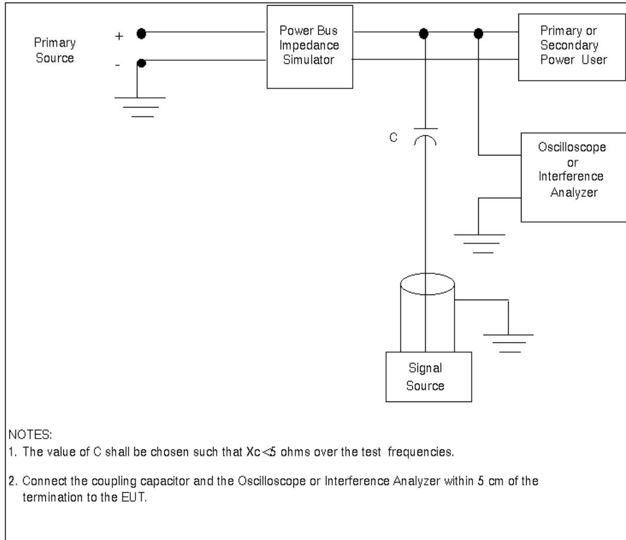
FIGURE 3.4.3.2.3-1 CS02 Test Setup for Equipment 160V Primary Power or 120 V Secondary Power
