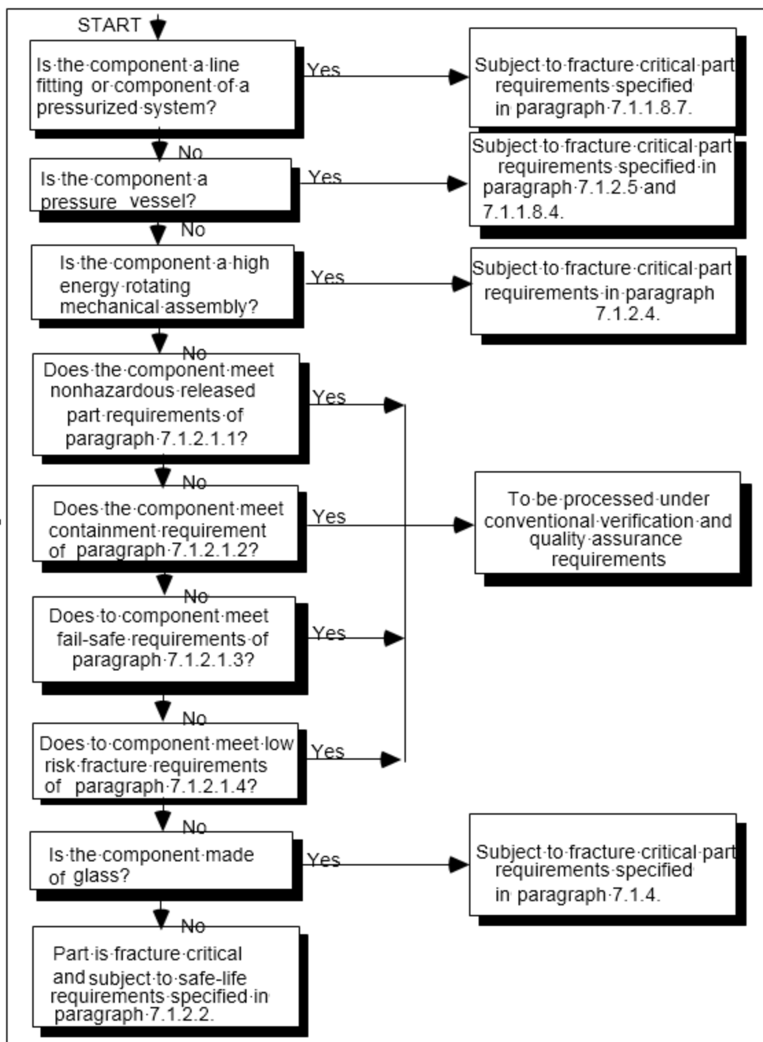
FIGURE 7.1.2.1-1 FRACTURE CONTROL CLASSIFICATION OF ISS COMPONENTS
