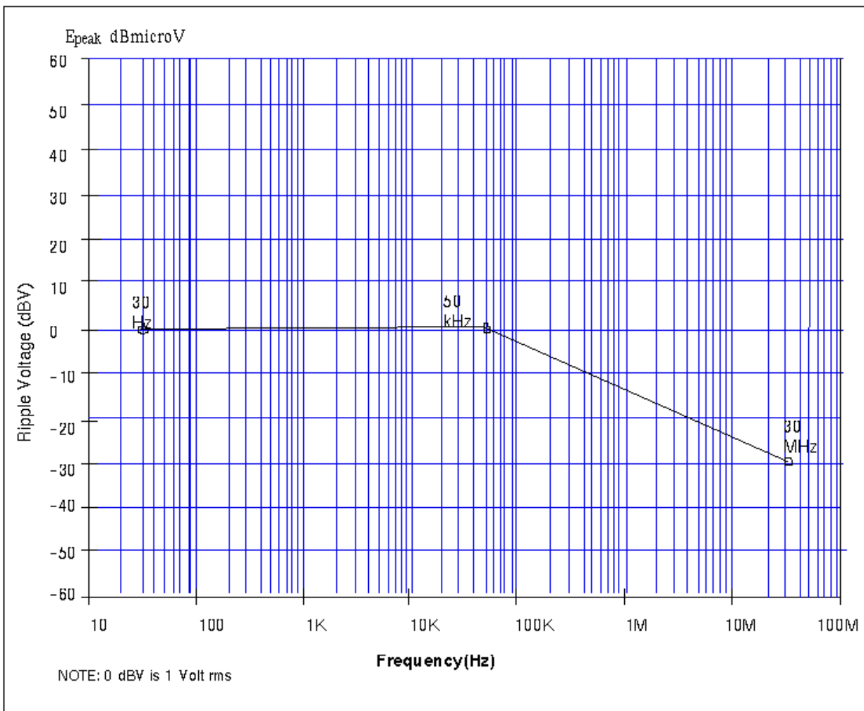
FIGURE 3.4.2.1.1.2-1 120 V SECONDARY BUS MAXIMUM VOLTAGE RIPPLE LIMITS (VOLTAGE SPECTRAL COMPONENTS)
