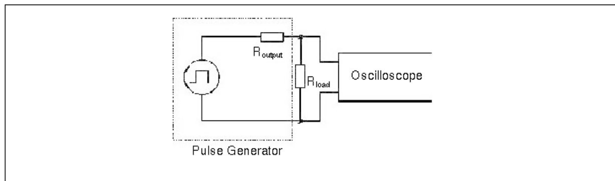
FIGURE 3.4.1.2.3-2 CALIBRATION OF PULSE GENERATOR
