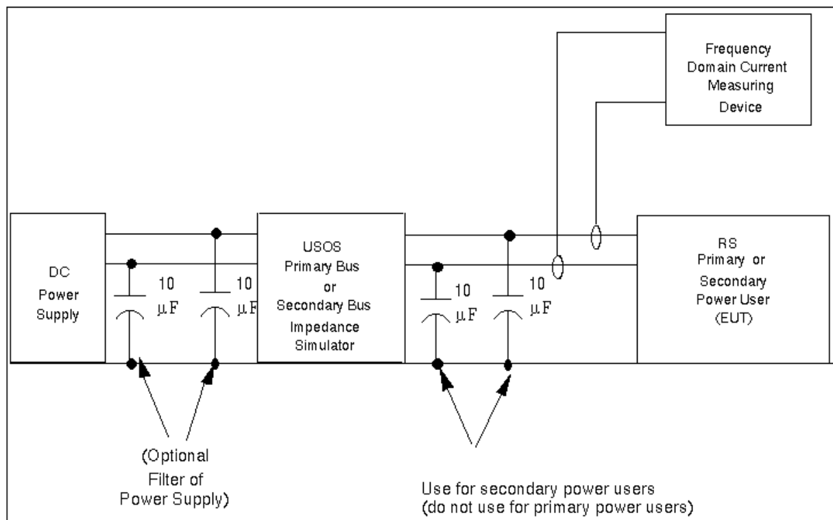
FIGURE 3.4.3.1.1-2 CONDUCTED EMISSIONS TEST SETUP FOR USOS PRIMARY POWER USERS AND USOS SECONDARY POWER USERS
