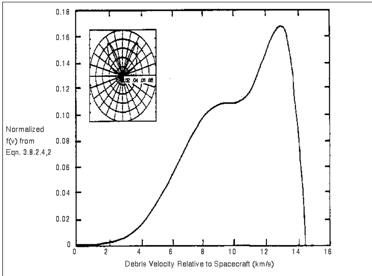
FIGURE 3.8.2.4-1 NORMALIZED COLLISION VELOCITY DISTRIBUTION AS FUNCTION OF THE DEBRIS VELOCITY FOR A SPACECRAFT WITH AN ORBITAL INCLINATION OF 28.5 DEGREES
