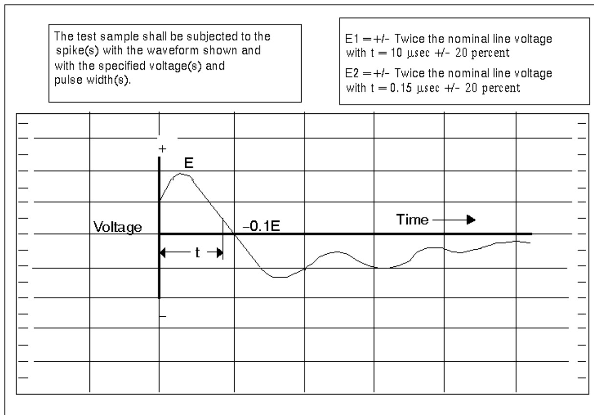
FIGURE 3.4.3.2.5-1 CONDUCTED SPIKE SUSCEPTIBILITY (CS06) LIMIT FOR EQUIPMENT USING THE USOS PRIMARY OR SECONDARY POWER
