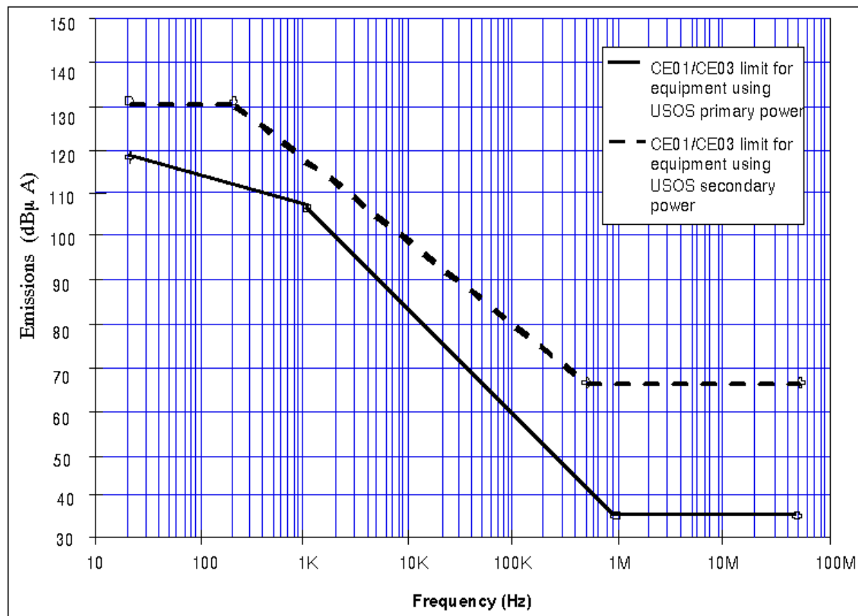
FIGURE 3.4.3.1.1-1 CONDUCTED EMISSION LIMIT (CE01/CE03) FOR EQUIPMENT USING 160V PRIMARY POWER AND FOR EQUIPMENT USING 120 V SECONDARY POWER
