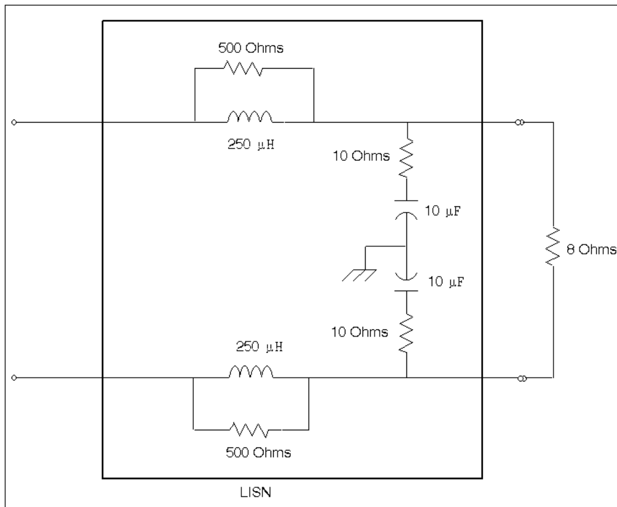
FIGURE 3.4.2.1.1-4 SECONDARY BUS LOAD IMPEDANCE EQUIVALENT NETWORK
