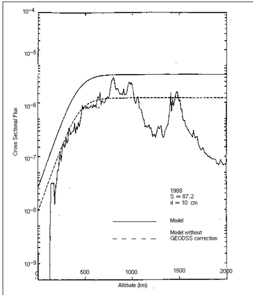
FIGURE 3.8.2.5.2-1 COMPARISON OF MODEL FLUX, F_c , WITH CATALOG FLUX NOT CORRECTED FOR GEODSS RESULTS
