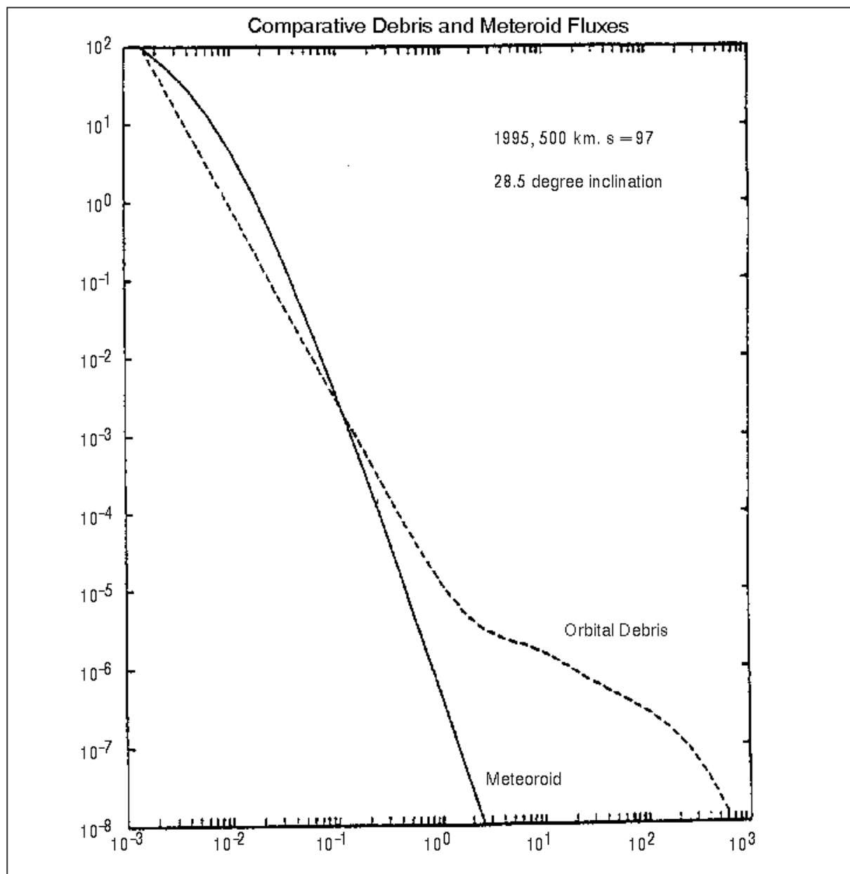
FIGURE 3.8.1-2 COMPARISON OF METEOROID AND ORBITAL DEBRIS FLUXES, F_r , AS A FUNCTION OF SIZE
