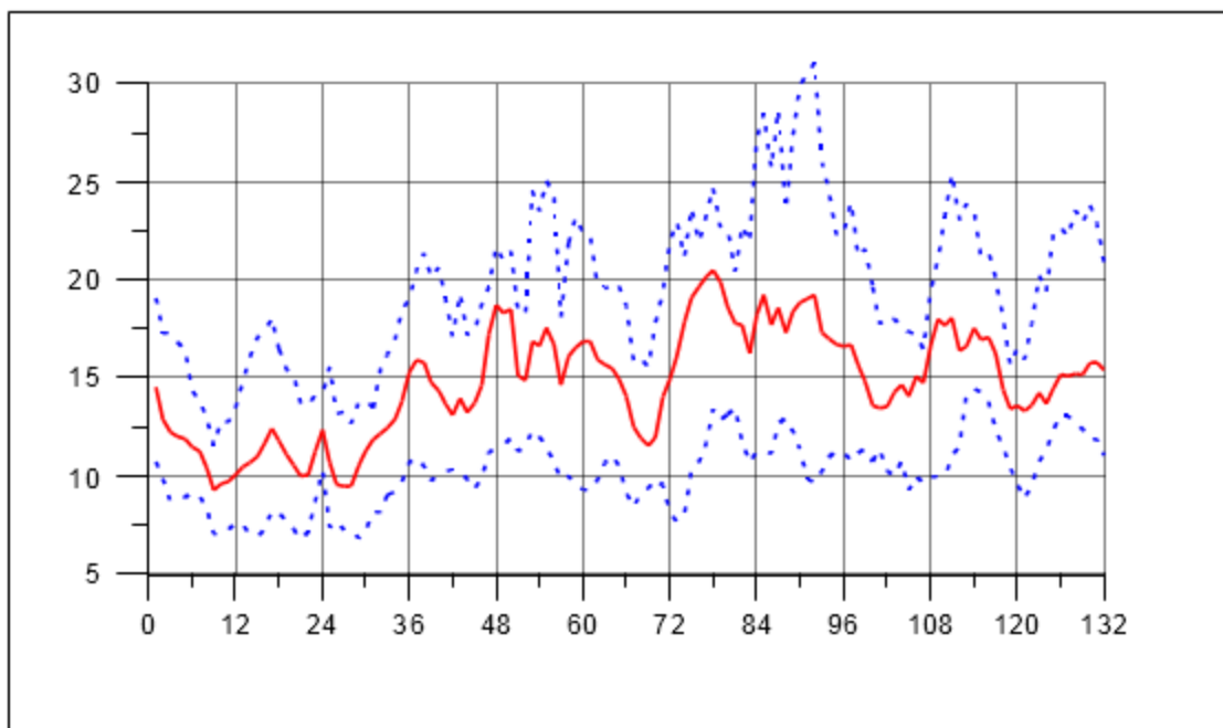
FIGURE 3.2.1.1-2 RSA FEB-96 DESIGN ATMOSPHERE PROFILE FOR SOLAR CYCLE 23: GEOMAGNETIC INDEX
