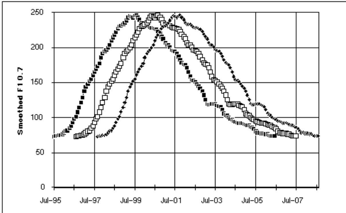
FIGURE 3.2.1.2-1 NASA DESIGN PROFILES FOR SOLAR CYCLE 23; F10.7 ASSUMING EARLY, MOST LIKELY, AND LATE START DATES
