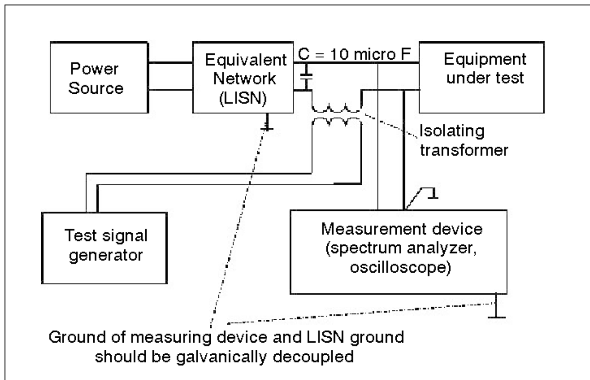
FIGURE 3.4.1.2.1-2 MODEL FOR TESTING OF EQUIPMENT FOR CONDUCTED INTERFERENCE IMMUNITY
