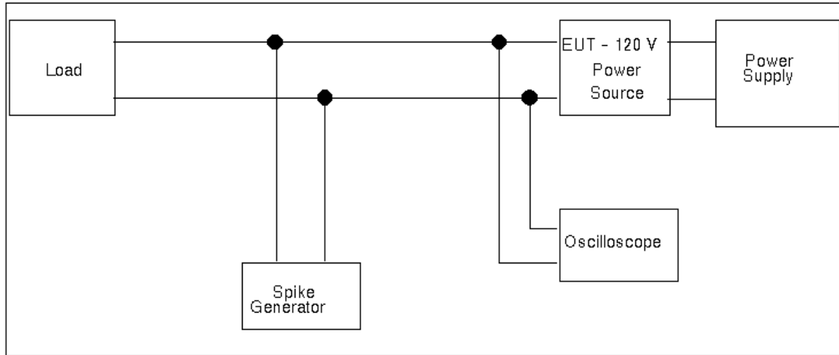
FIGURE 3.4.2.2.4-3 CONDUCTED SPIKE SUSCEPTIBILITY (CS06) PARALLEL INJECTION TEST SETUP FOR EQUIPMENT PROVIDING POWER TO THE USOS
