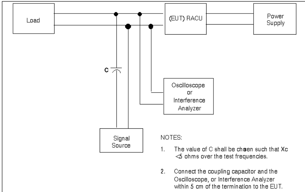
FIGURE 3.4.2.2.3-1 CONDUCTED SUSCEPTIBILITY (CS02) TEST SETUP FOR EQUIPMENT PROVIDING USOS POWER
