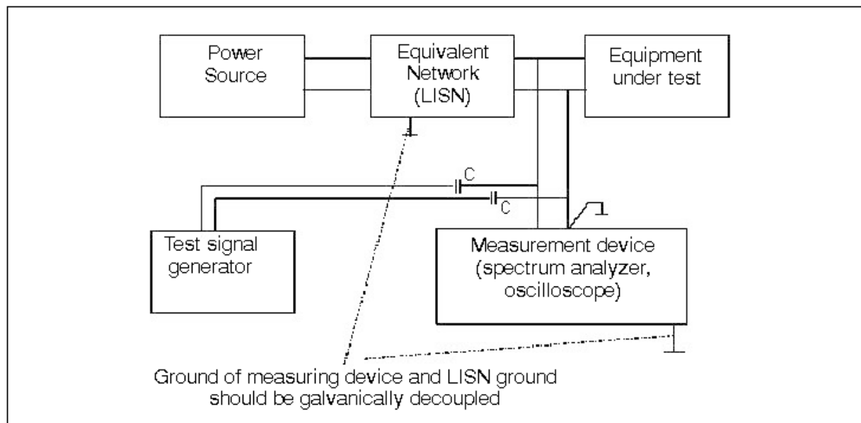
FIGURE 3.4.1.2.2-2 EQUIPMENT TEST SETUP FOR INTERFERENCE IMMUNITY IN POWER LINES
