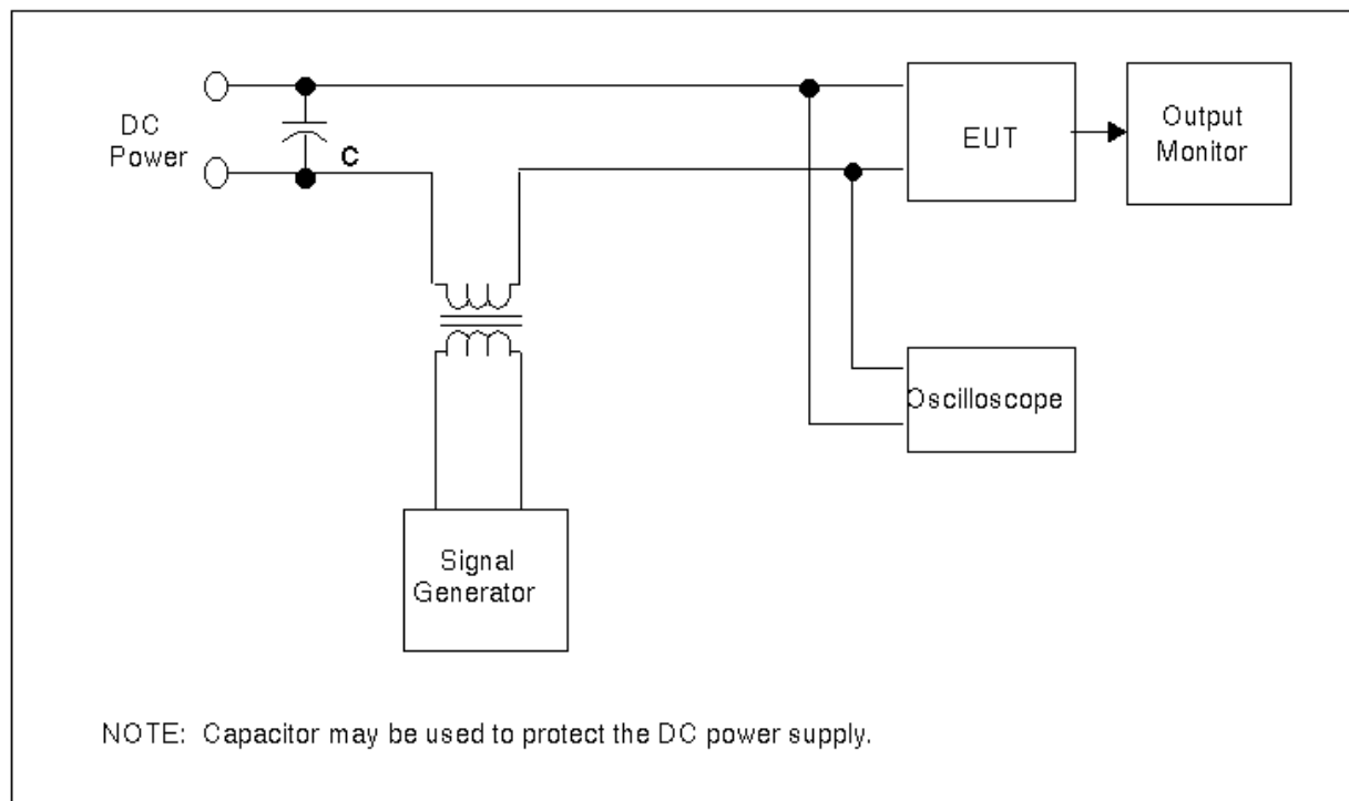
FIGURE 3.4.3.2.5-2 CONDUCTED SPIKE SUSCEPTIBILITY (CS06) SERIES INJECTION TEST SETUP FOR EQUIPMENT USING THE USOS PRIMARY OR SECONDARY POWER
