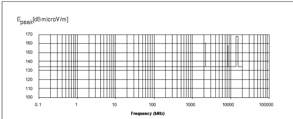
FIGURE 3.4.1.2.5-1 EQUIPMENT IMMUNITY REQUIREMENTS (INTENSITY OF THE ELECTRICAL FIELD OUTSIDE AN OBJECT)
