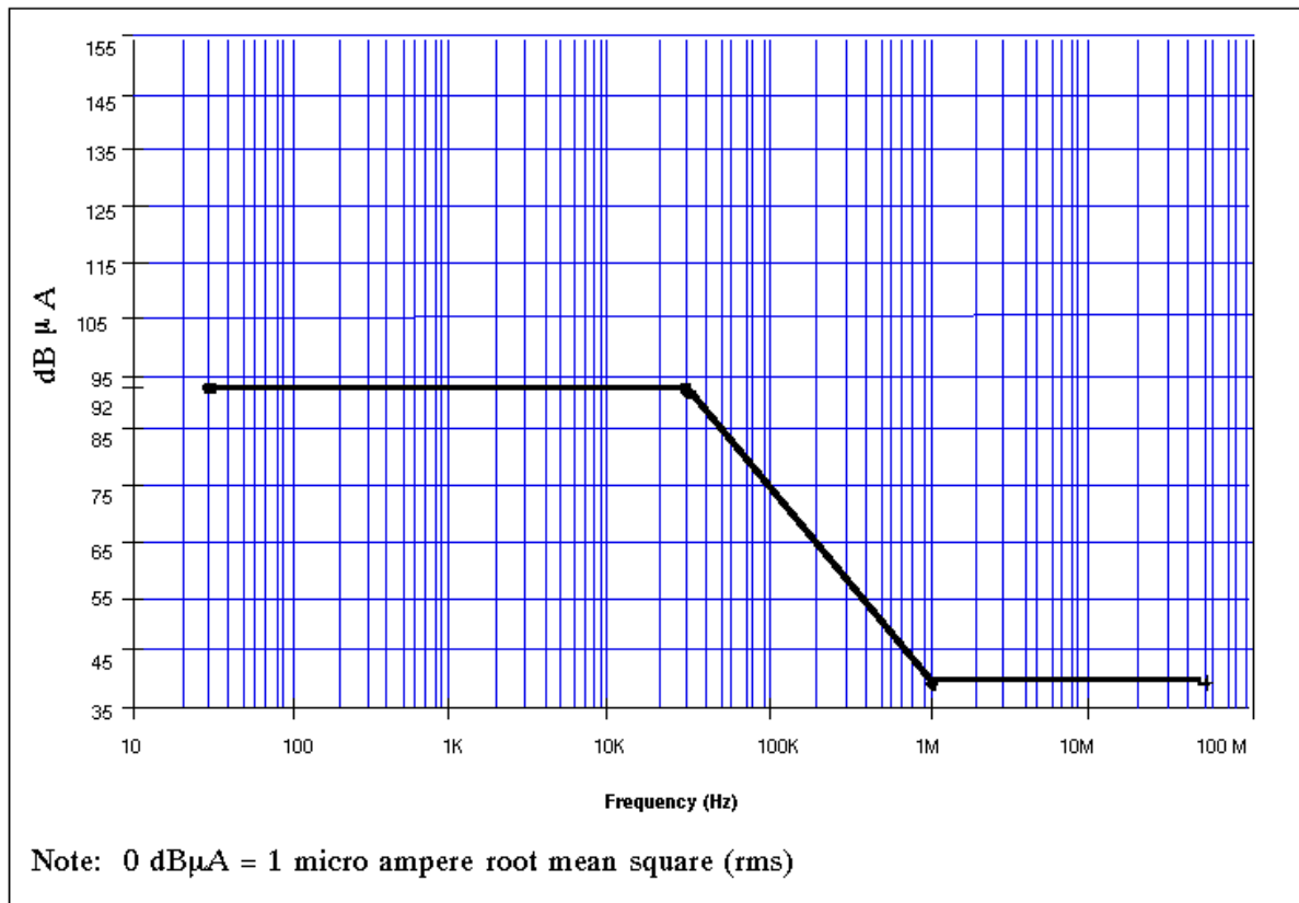
FIGURE 3.4.2.1.1-1 CONDUCTED EMISSIONS LIMIT (CE01/CE03) FOR EQUIPMENT PROVIDING POWER TO USOS
