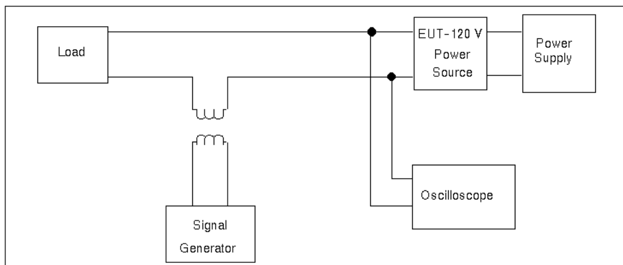
FIGURE 3.4.2.2.4-2 CONDUCTED SPIKE SUSCEPTIBILITY, (CS06) SERIES INJECTION TEST SETUP FOR EQUIPMENT PROVIDING POWER TO THE USOS
