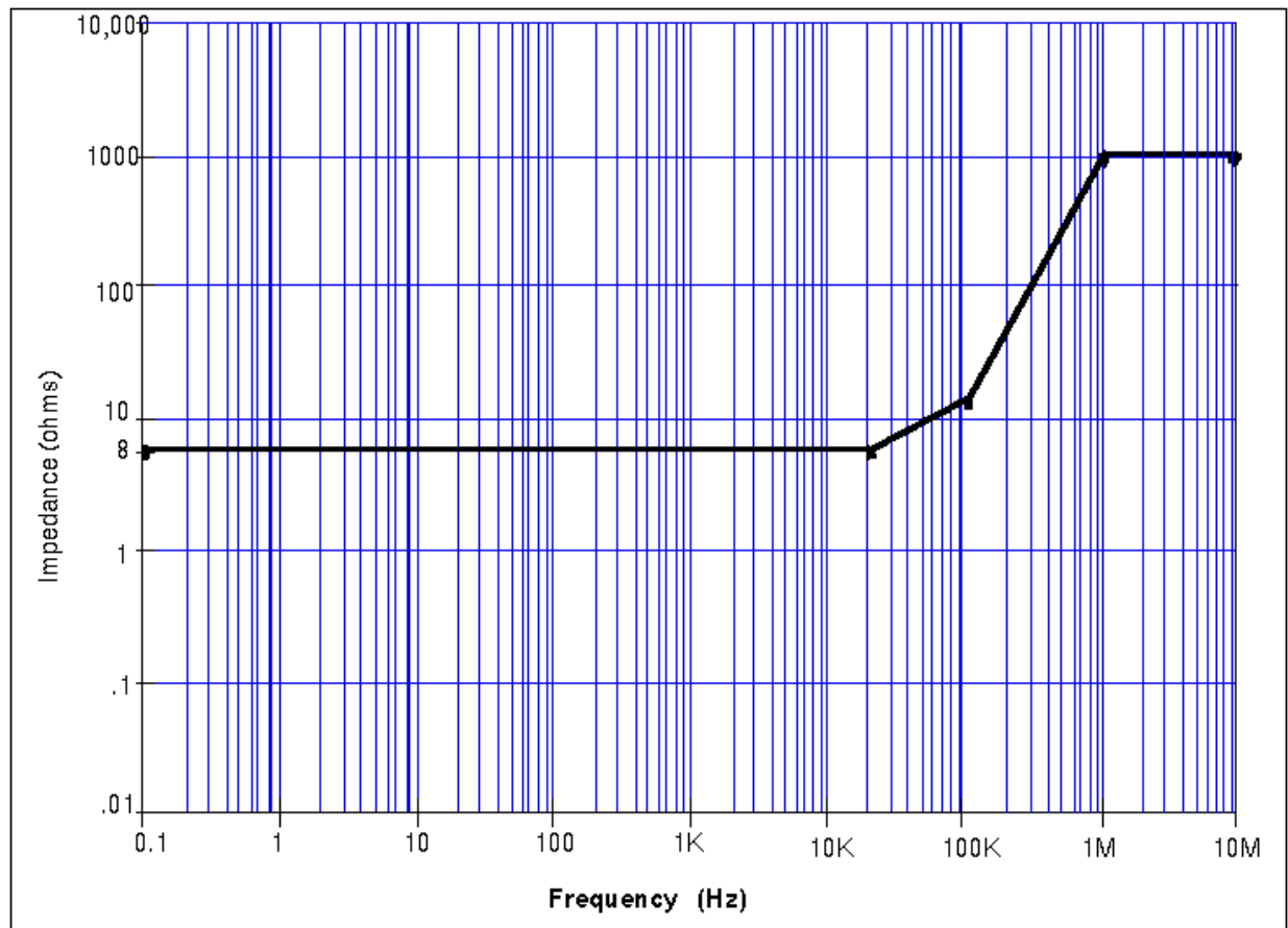
FIGURE 3.4.2.1.1-3 SECONDARY BUS LOCAL IMPEDANCE
