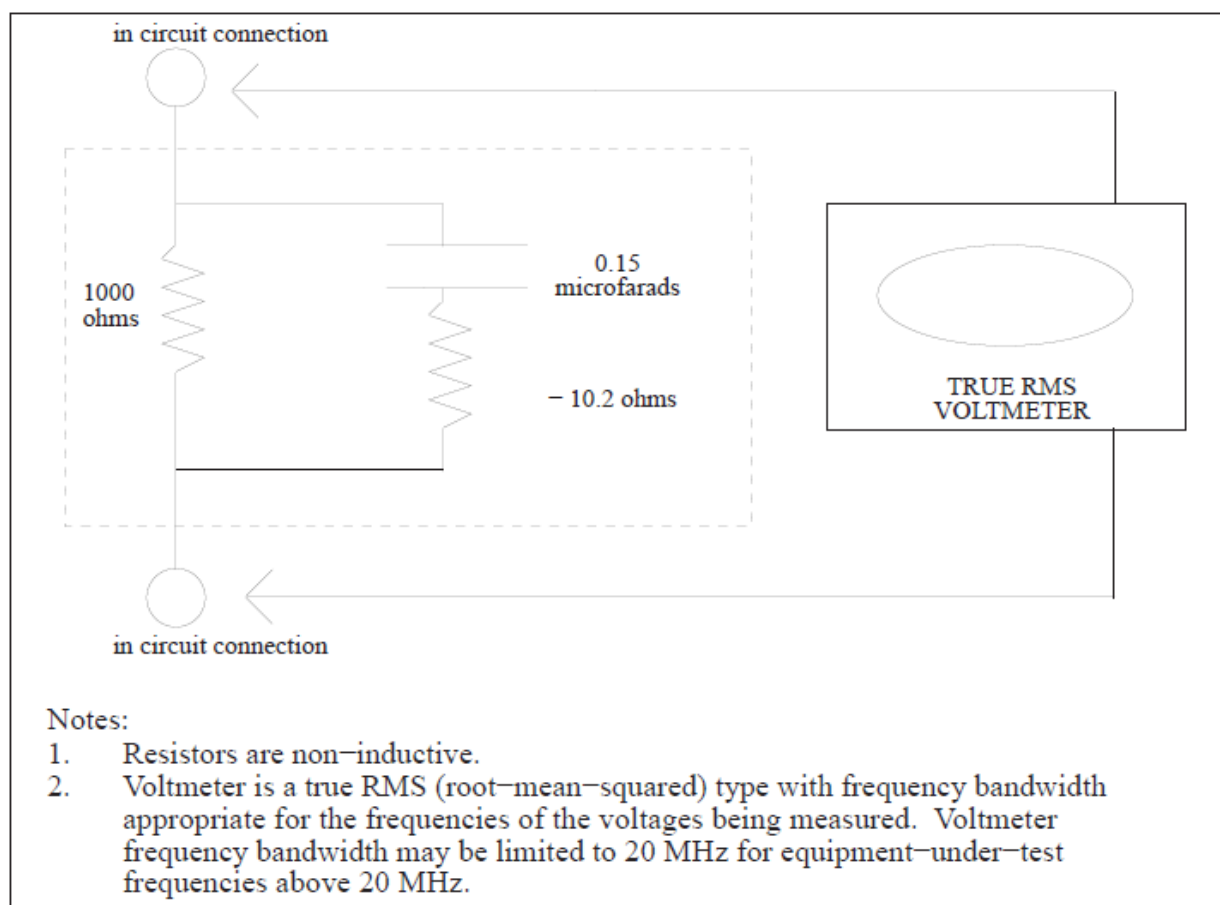
FIGURE 6.5.1.15-1 LEAKAGE CURRENT VERIFICATION NETWORK
