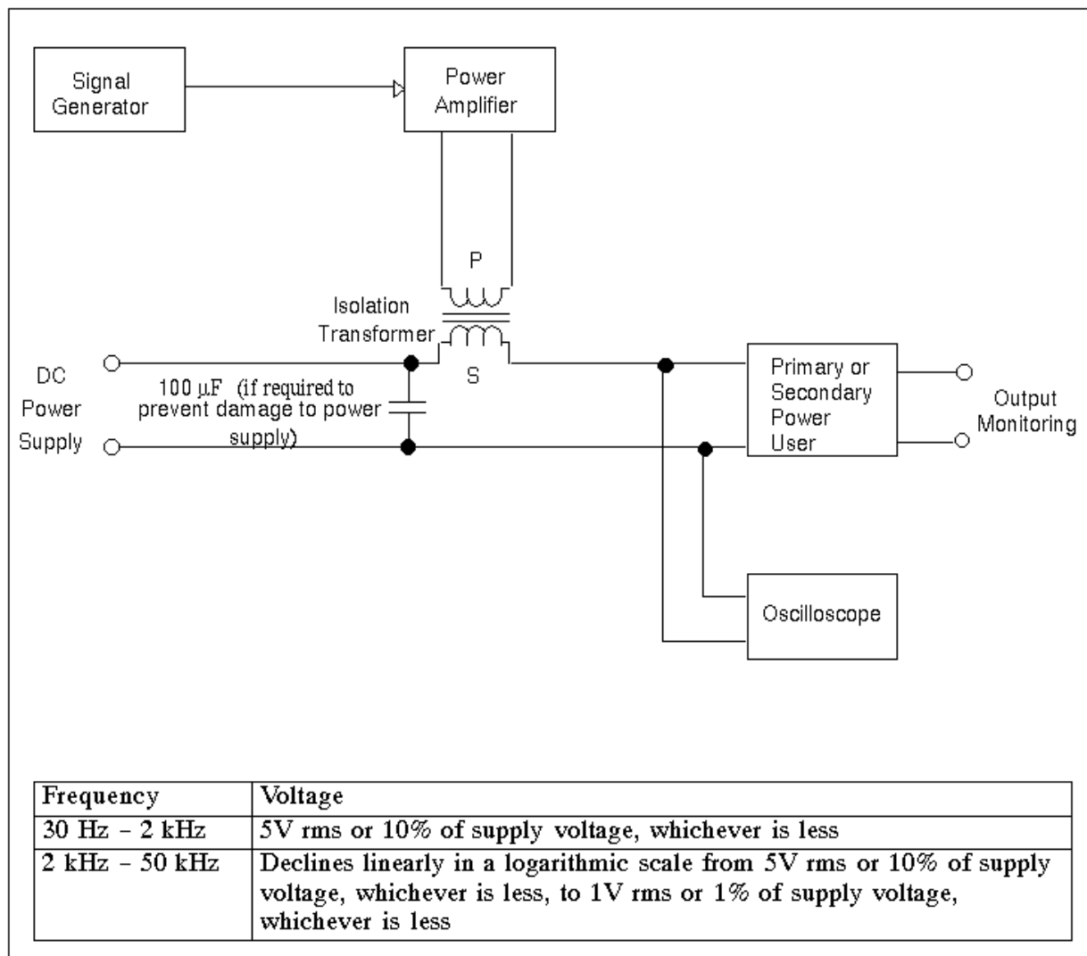
FIGURE 3.4.3.2.1-2 CS01 TEST SETUP FOR EQUIPMENT USING USOS PRIMARY OR SECONDARY POWER
