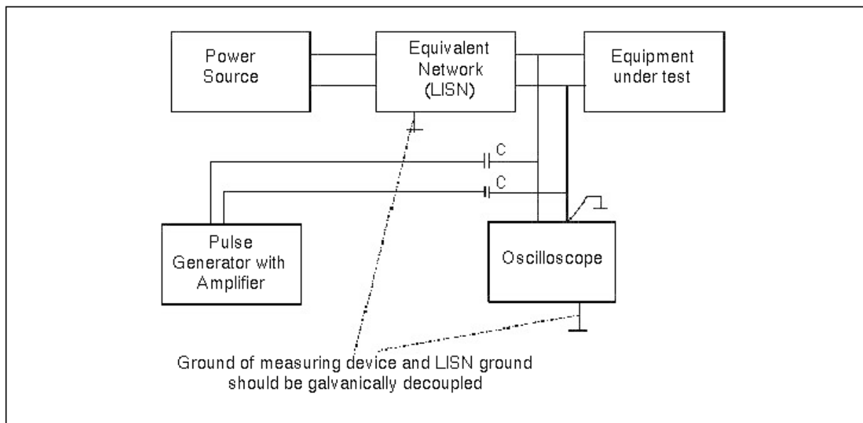
FIGURE 3.4.1.2.3-1 MODEL FOR TESTING OF EQUIPMENT FOR CONDUCTED PULSE INTERFERENCE IMMUNITY
