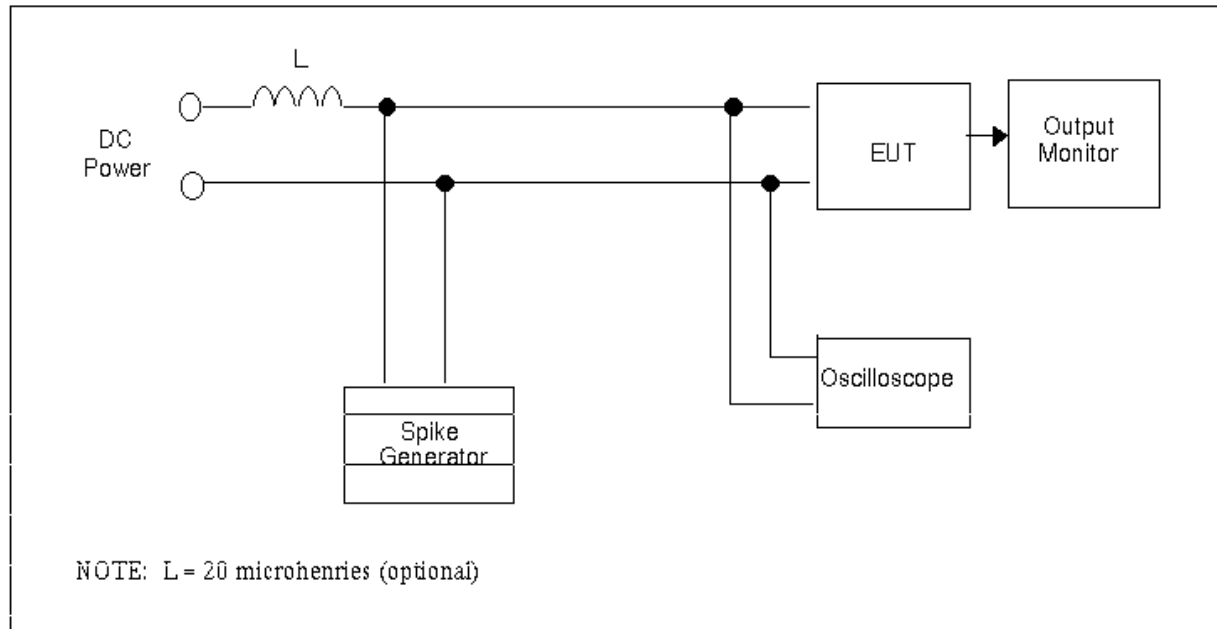
FIGURE 3.4.3.2.5-3 CONDUCTED SPIKE SUSCEPTIBILITY (CS06) PARALLEL INJECTION TEST SETUP FOR EQUIPMENT USING THE USOS PRIMARY OR SECONDARY POWER
