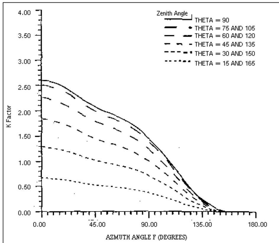
FIGURE 3.8.3-1 "K" FACTOR FOR SINGLE SIDED FLAT PLATES
