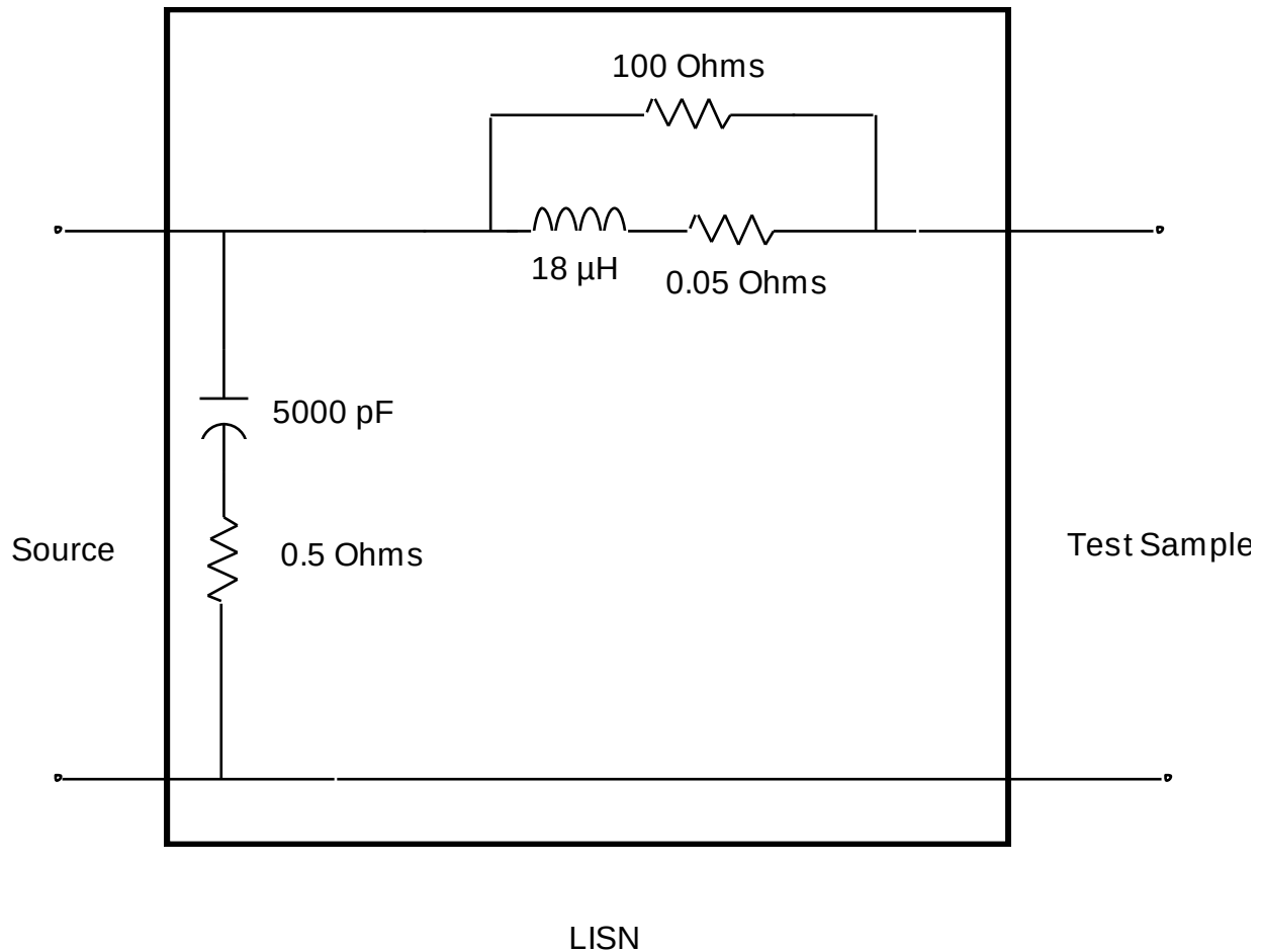
FIGURE 3.4.3.1.1-5 USOS SECONDARY POWER BUS EQUIVALENT NETWORK
