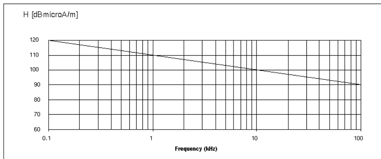
FIGURE 3.4.1.2.4-1 EQUIPMENT IMMUNITY REQUIREMENTS (INTENSITY OF THE MAGNETIC FIELD INSIDE A MODULE)
