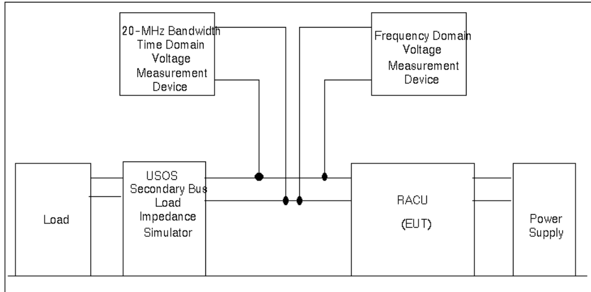
FIGURE 3.4.2.1.1.1-1 120 V SECONDARY POWER SOURCE VOLTAGE RIPPLE TEST SETUP
