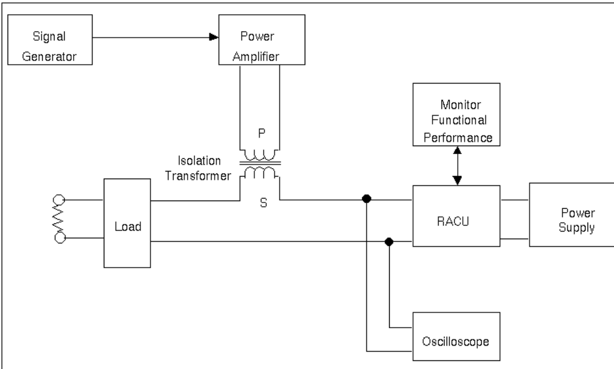
FIGURE 3.4.2.2.2-1 CONDUCTED SUSCEPTIBILITY (CS01) TEST SETUP FOR EQUIPEMENT PROVIDING POWER FOR THE USOS
