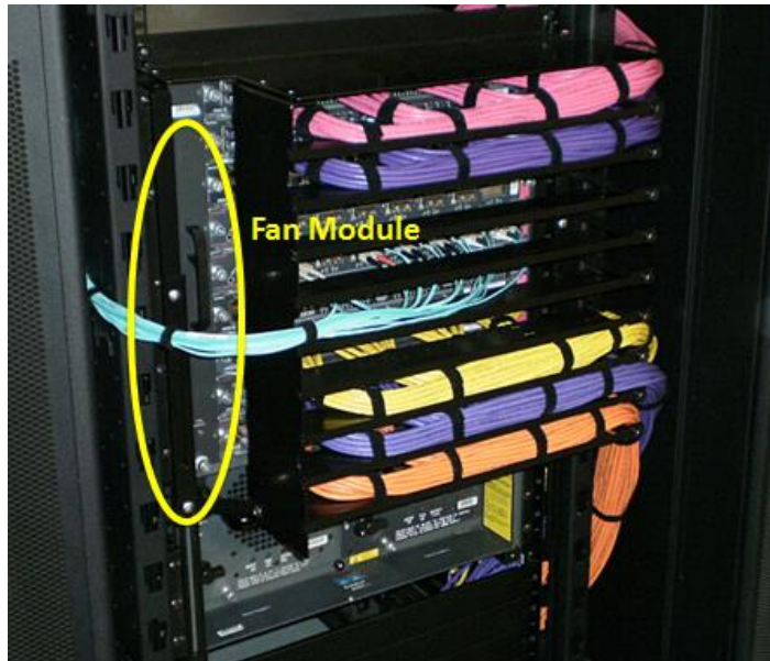
Figure 20: Equipment-Specific Cable Management Requirements
