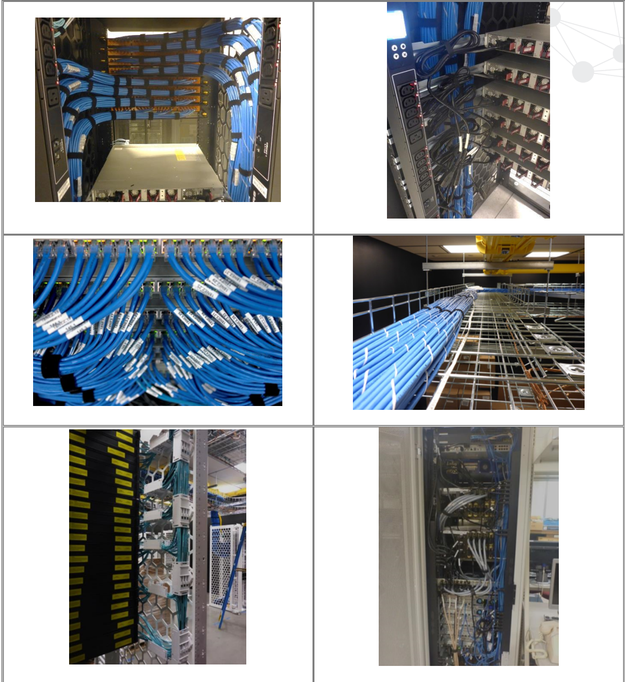
Figure 21: Acceptable Cable Management Results
