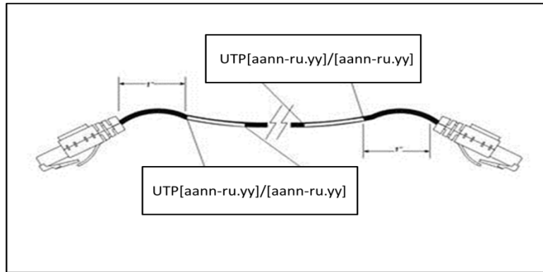
Figure 18: Detailed Example of Communications Cable Labeling
