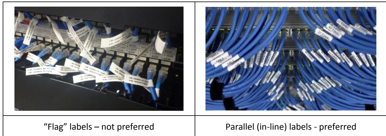
Figure 17: Example of Communications Cable Labeling
