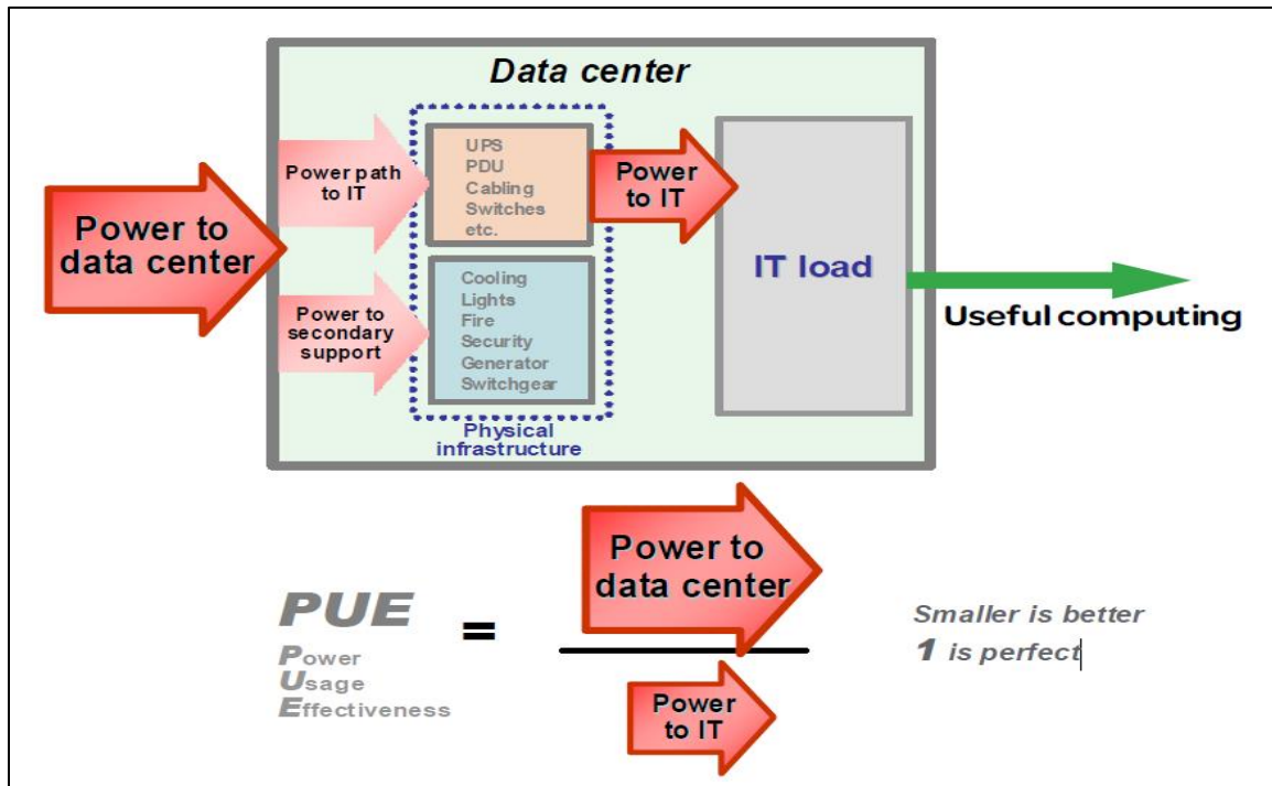
Figure 13: Power Utilization Effectiveness (PUE)
