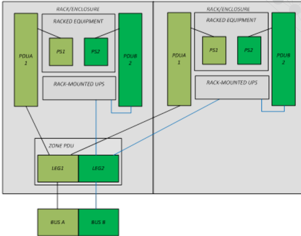
Figure 12: TR Topology with In-Rack UPS Backup (NSC)
