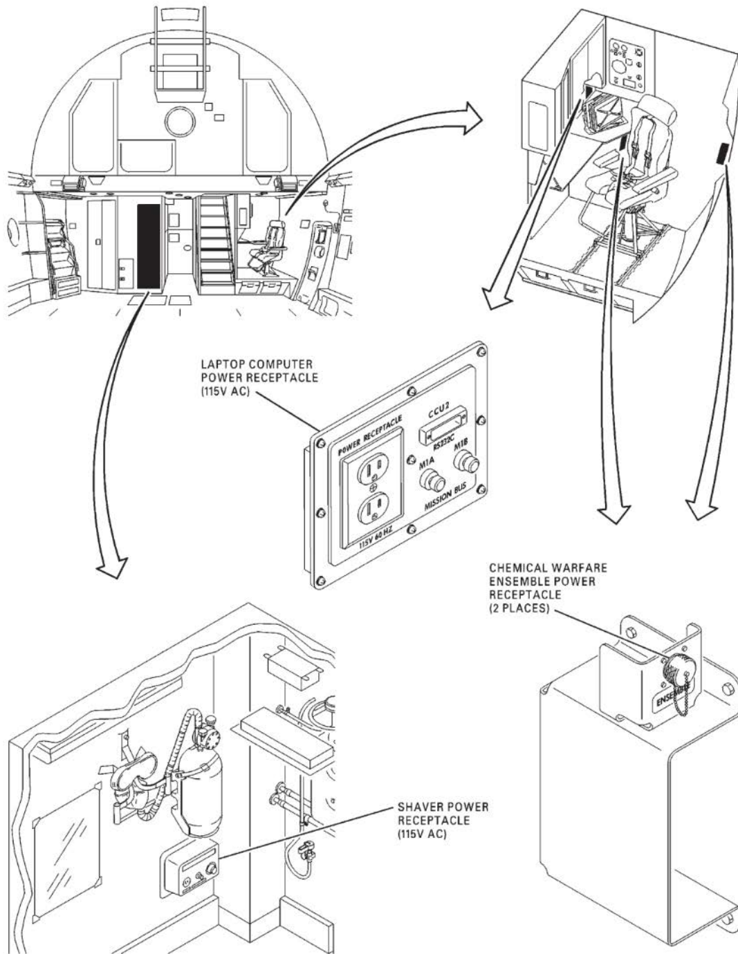
FIGURE B-76. Cargo compartment electrical receptacles.
