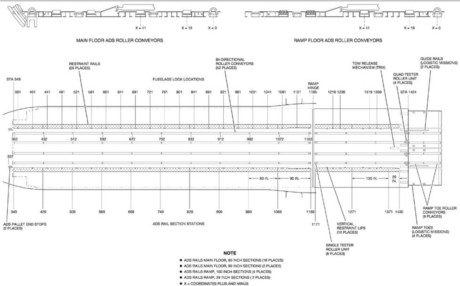
FIGURE B-67. C-17 ADS system - Continued (sheet 2 of 2).
