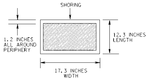
FIGURE B-34. Concentrated cargo maximum allowable floor loads (sheet 3 of 3).
