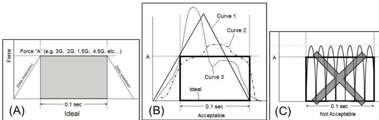
FIGURE A-24. Applied force curves.
