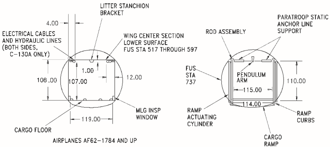
FIGURE B-80.a C-130 E/H cargo compartment dimensions.
