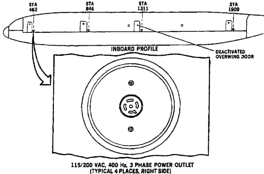
FIGURE B-123. Cargo compartment electrical outlets.
