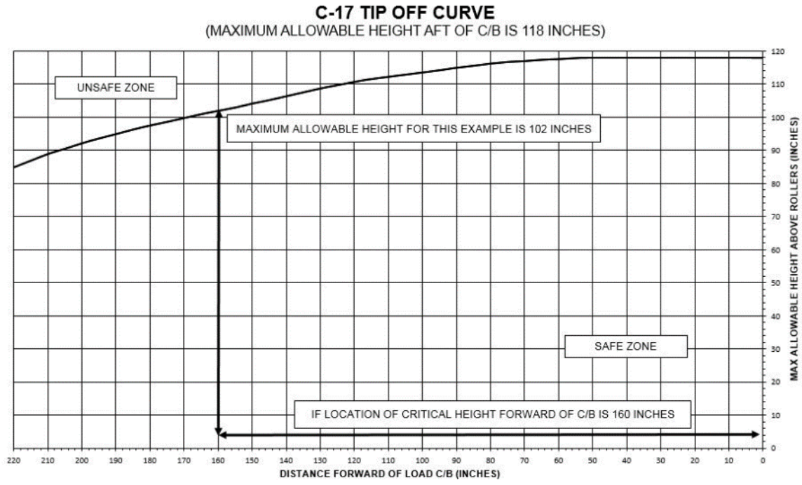
FIGURE B-77. C-17 tip off curve.
