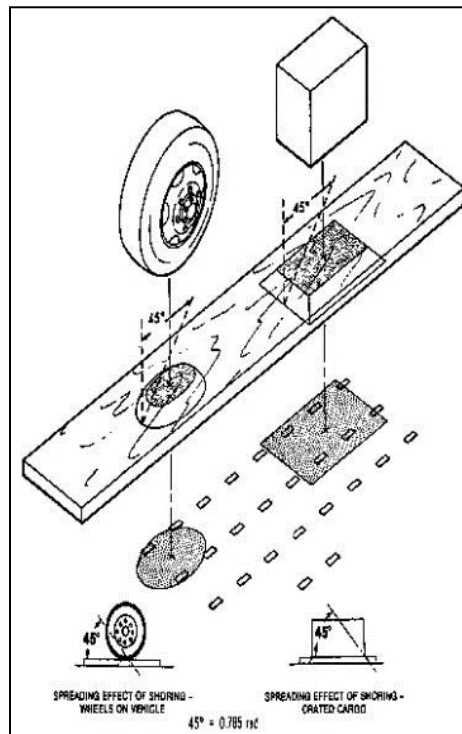
FIGURE A-42. Shoring to spread weight.
