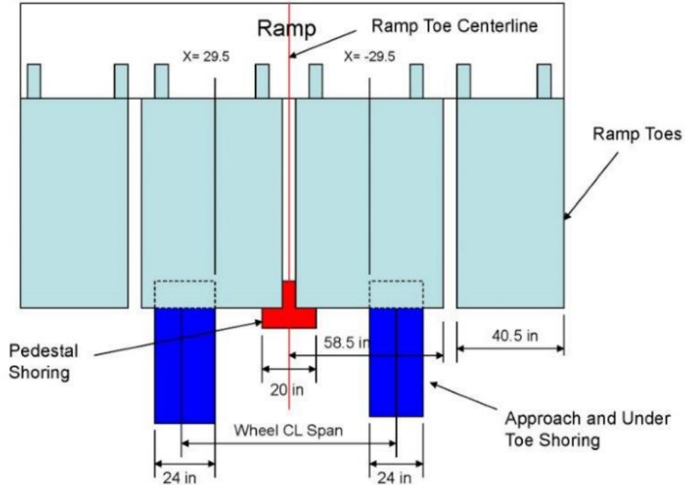
FIGURE B-59. C-17 minimum approach shoring width under ramp toes - (sheet 3 of 4).
