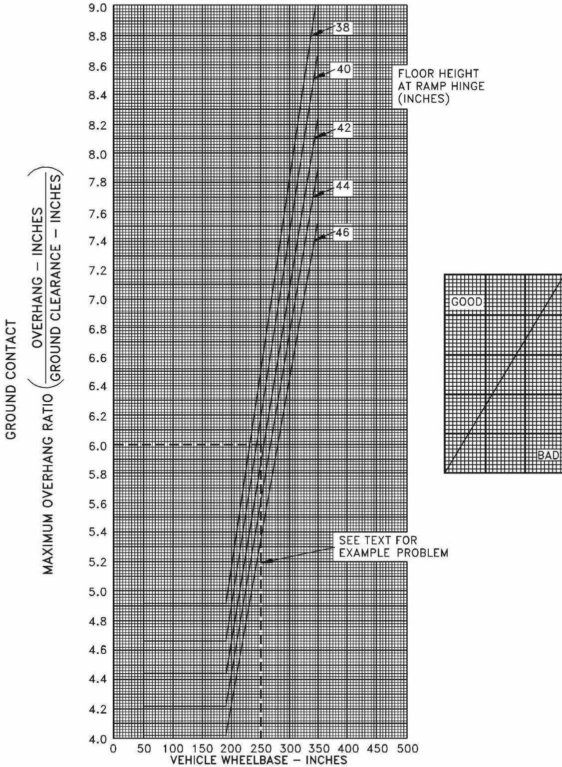
FIGURE B-87. Overhang and projection limits (vehicle).
