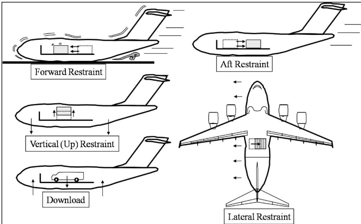
FIGURE A-22. Restraint for various situations.
