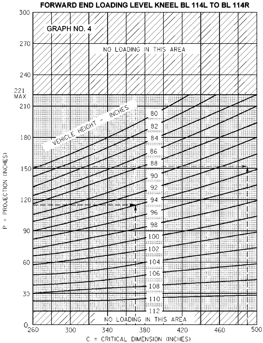
FIGURE B-13. Forward and aft end loading - vehicle projection limits.
