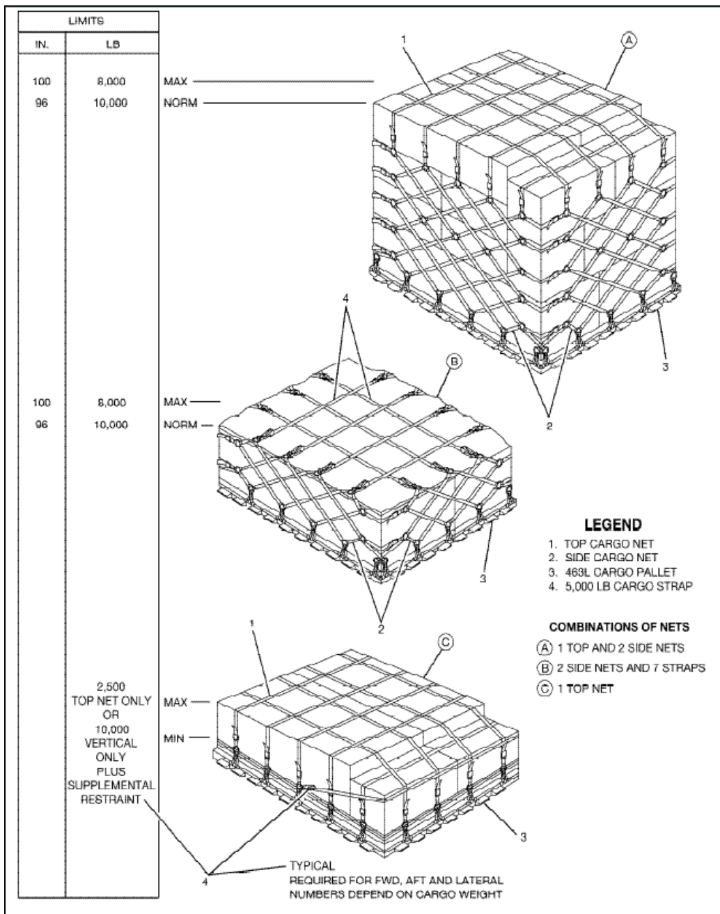
FIGURE A-9. Pallet size and weight limits with net restraint.
