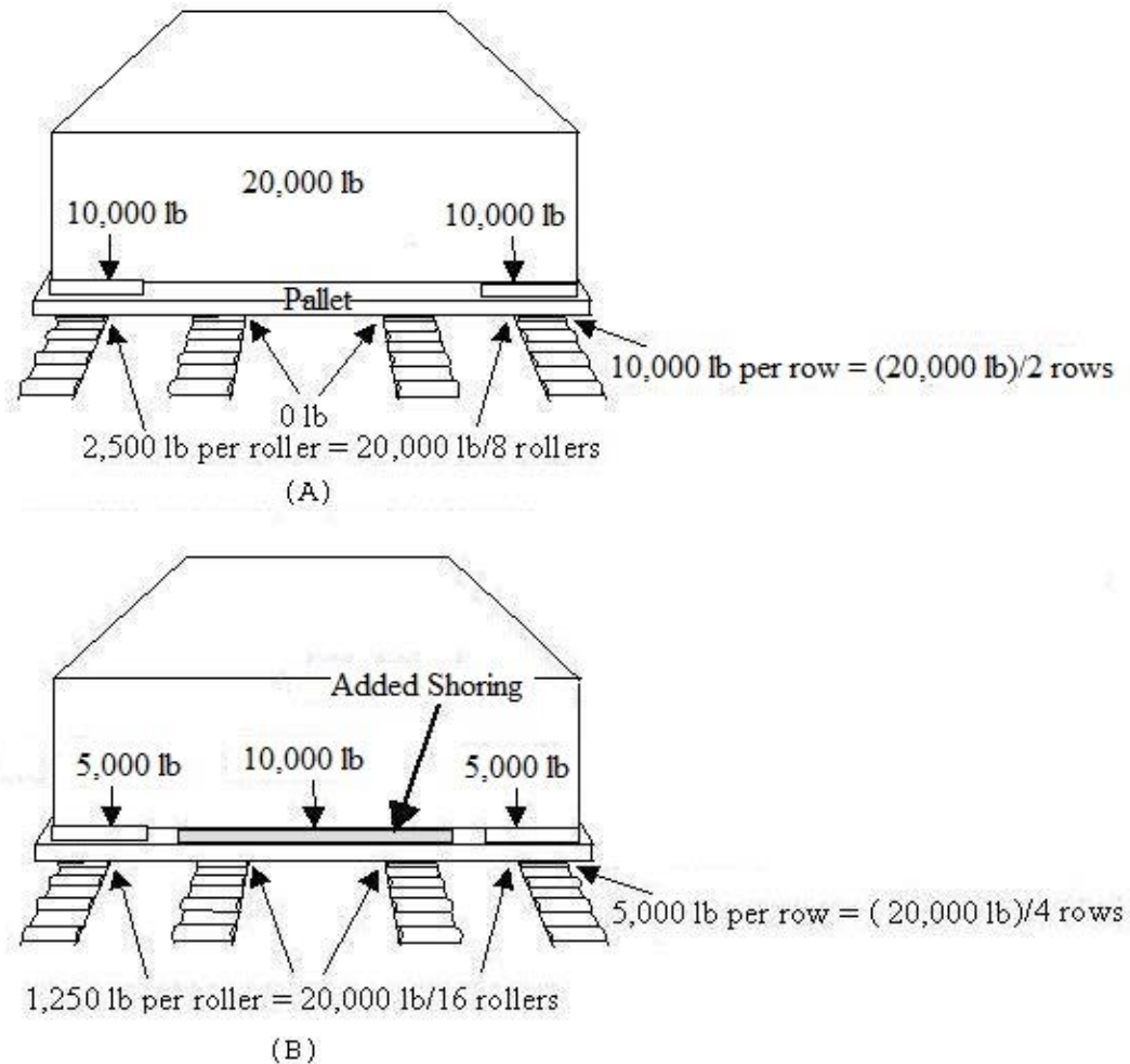
FIGURE A-16. Pallet/roller weight distribution.
