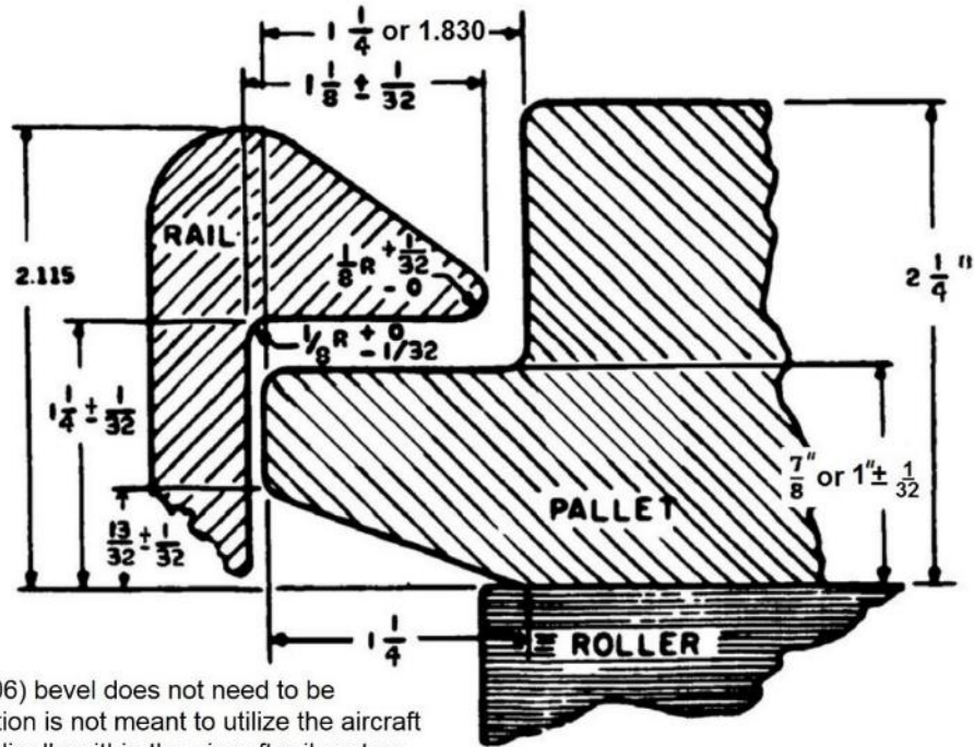
FIGURE 5. Pallet rail exterior profile.
