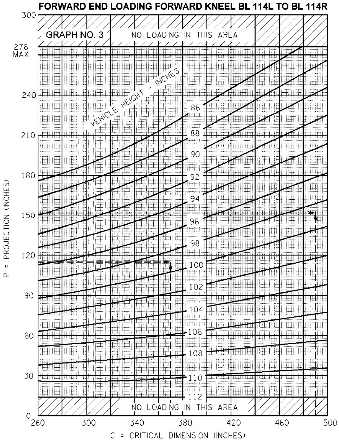
FIGURE B-12. Forward and aft end loading - vehicle projection limits.
