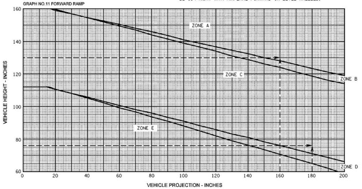
FIGURE B-20. Forward and aft end loading - vehicle projection limits.
