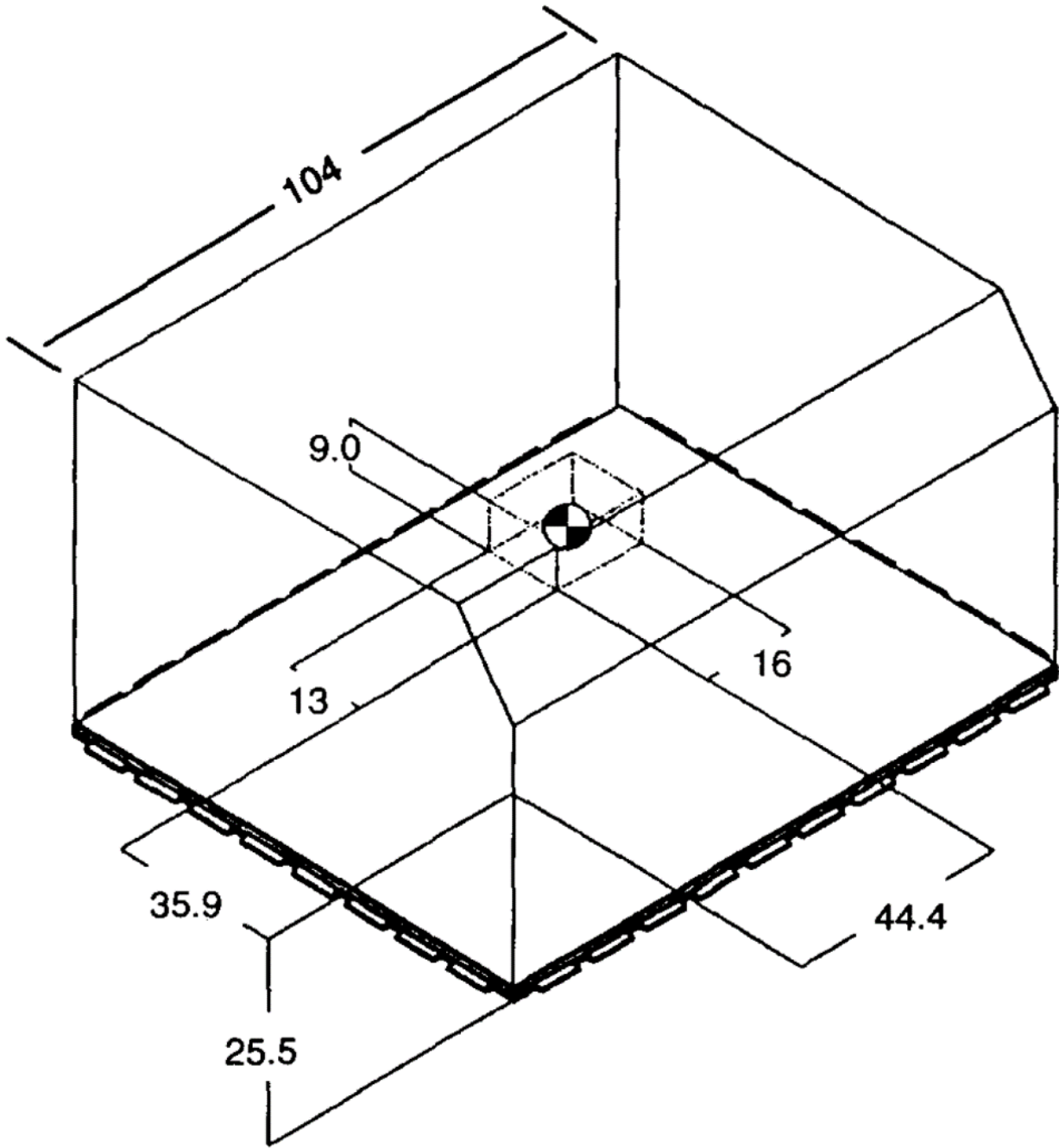
FIGURE B-134. KC-135 pallet CG requirements.
