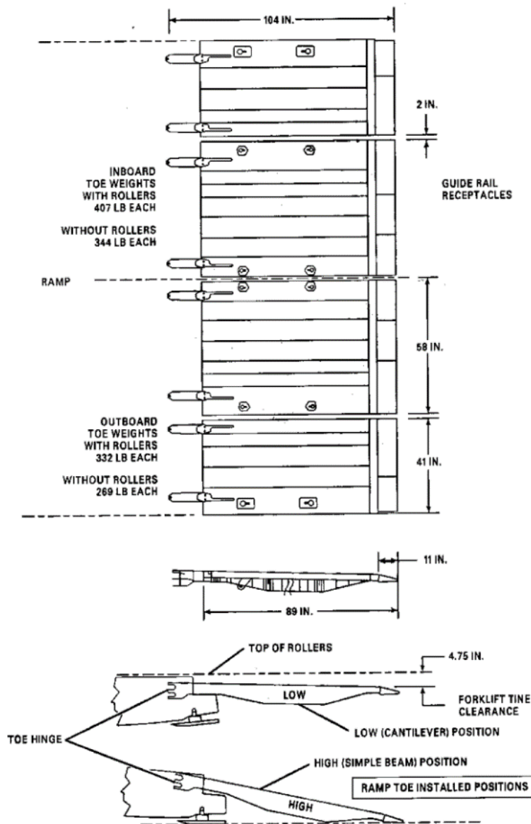
FIGURE B-69. Ramp toes.
