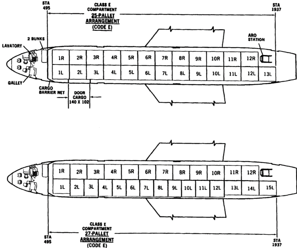
FIGURE B-113. All-cargo configuration.
