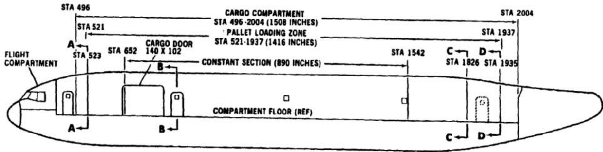
FIGURE B-107. Cargo compartment envelope.
