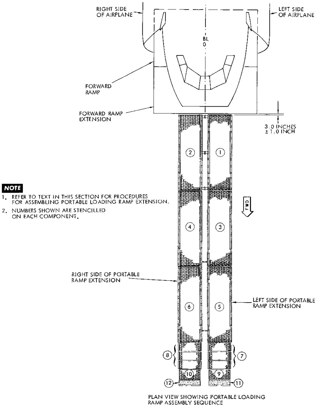
FIGURE B-31. Portable loading ramp extension assembly sequence.
