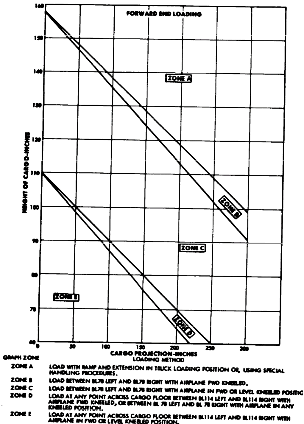
FIGURE B-7. Crated cargo projection limits (forward and aft end loading palletized) - Continued.
