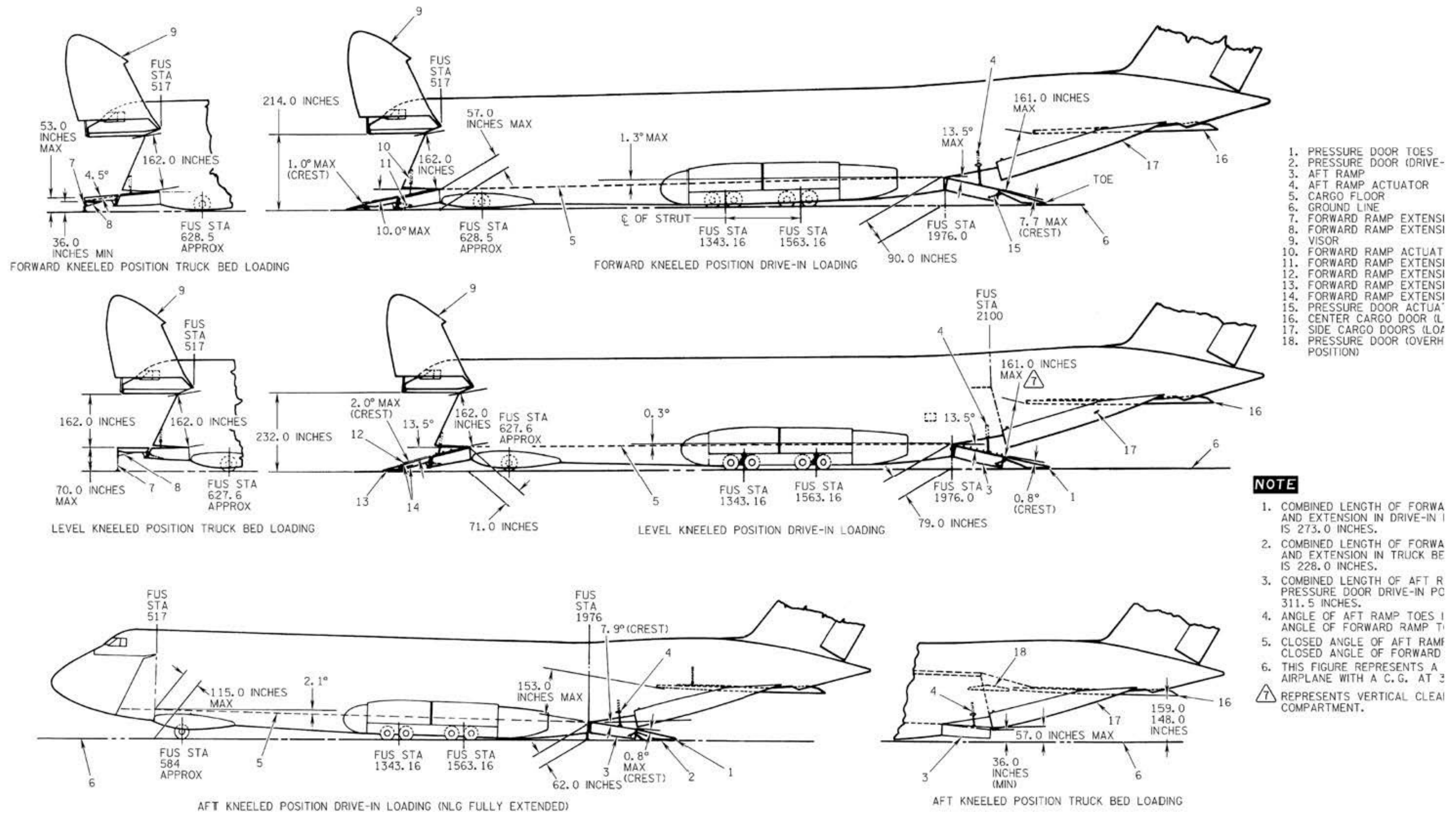
FIGURE B-6. Airplane kneeling loading position (on/off loading) - Continued.
