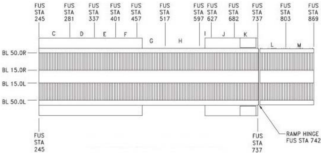
FIGURE B-90. Floor loading capacity - concentrated or pneumatic tire loads - Continued.
