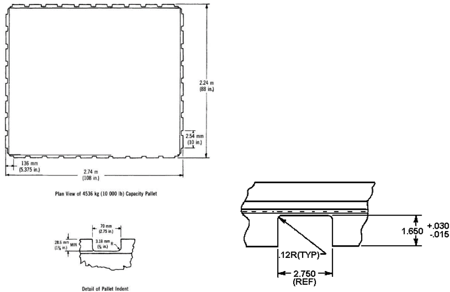
FIGURE A-8. Pallet and side rail.
