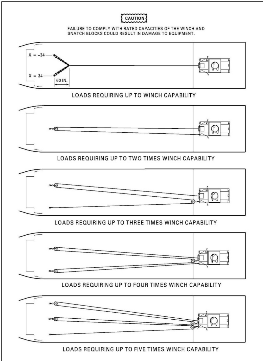
FIGURE A-51. Self-winch using snatch blocks.
