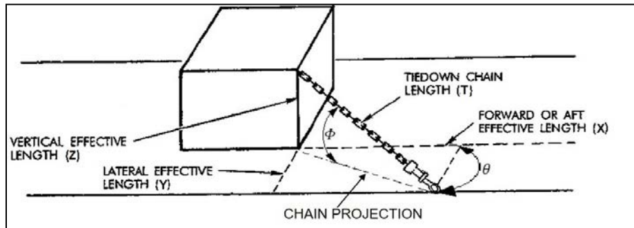
FIGURE A-27. Tiedown angles 1.
