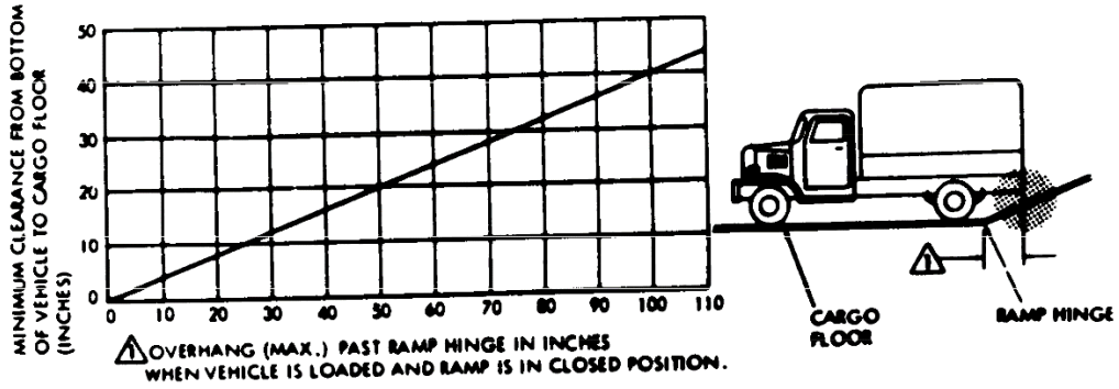
CHART B - PARKING OVERHANG LIMITS
