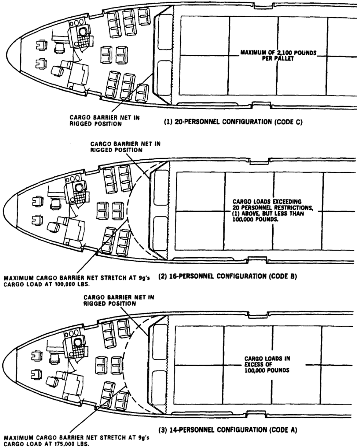
FIGURE B-109. Mixed cargo/personnel configuration.
