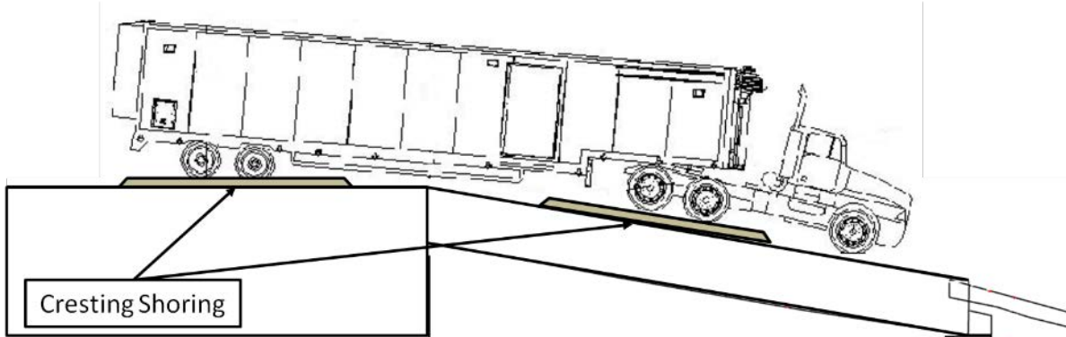
FIGURE A-41. Crestring shoring.
