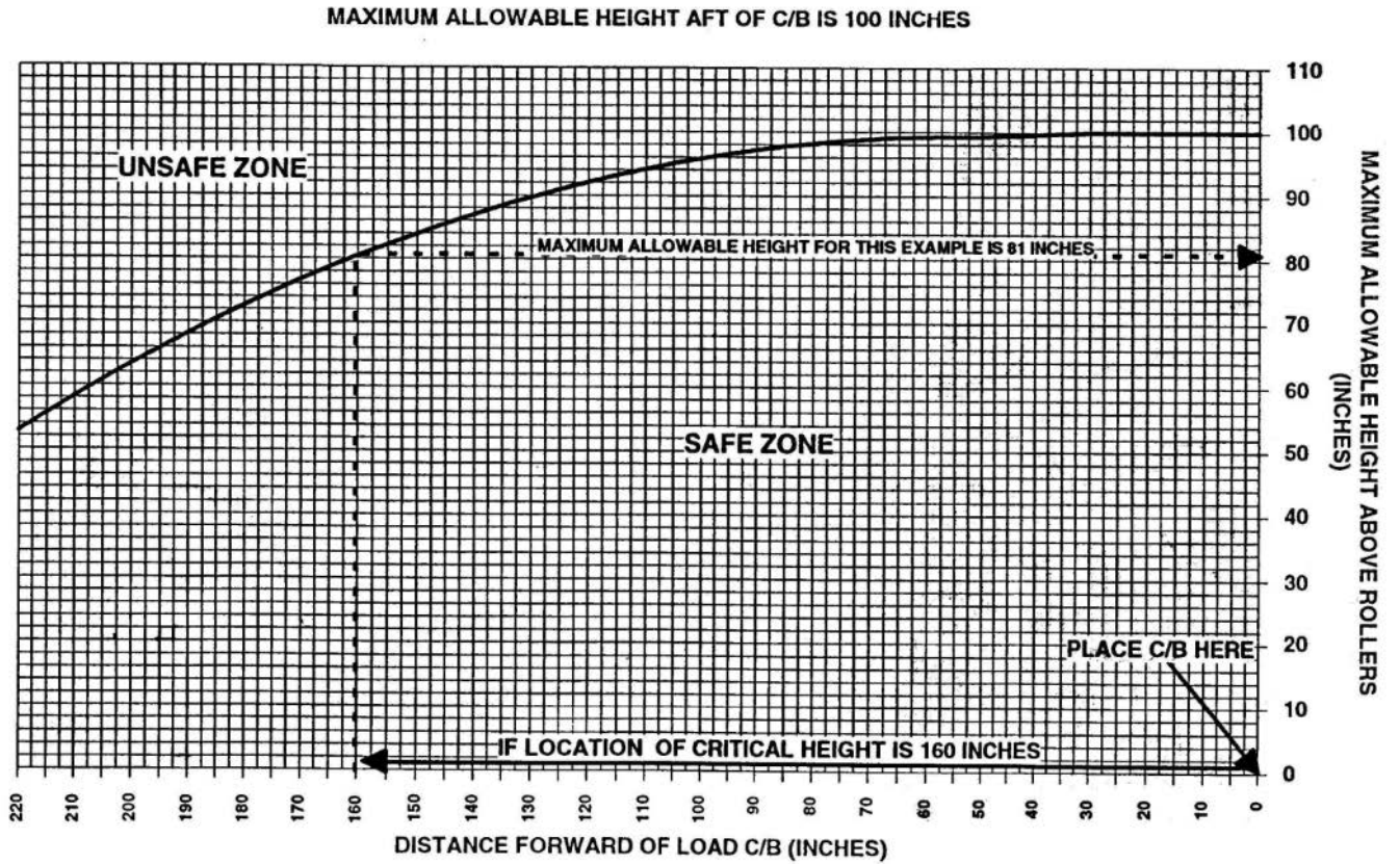
FIGURE B-103. C-130 tip off or jettison height limit curve (all variants).
