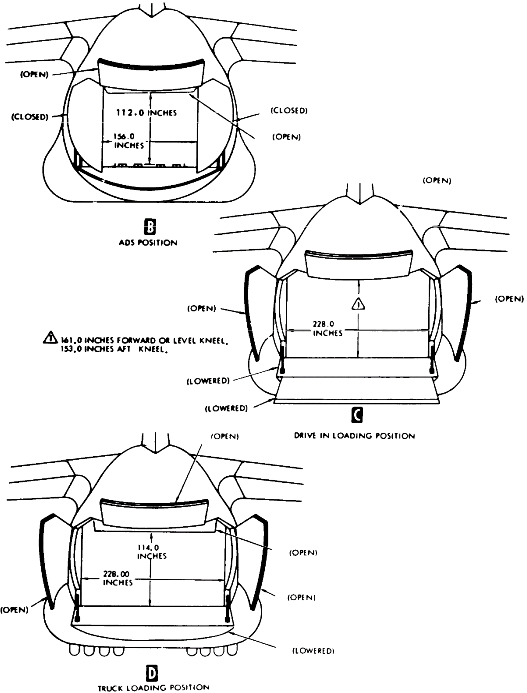
FIGURE B-4. Aft cargo opening dimensions.
