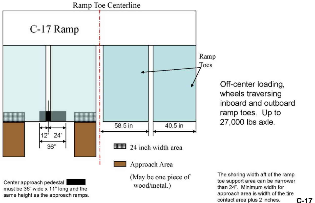
FIGURE B-59. C-17 minimum approach shoring width under ramp toes - (sheet 4 of 4).
