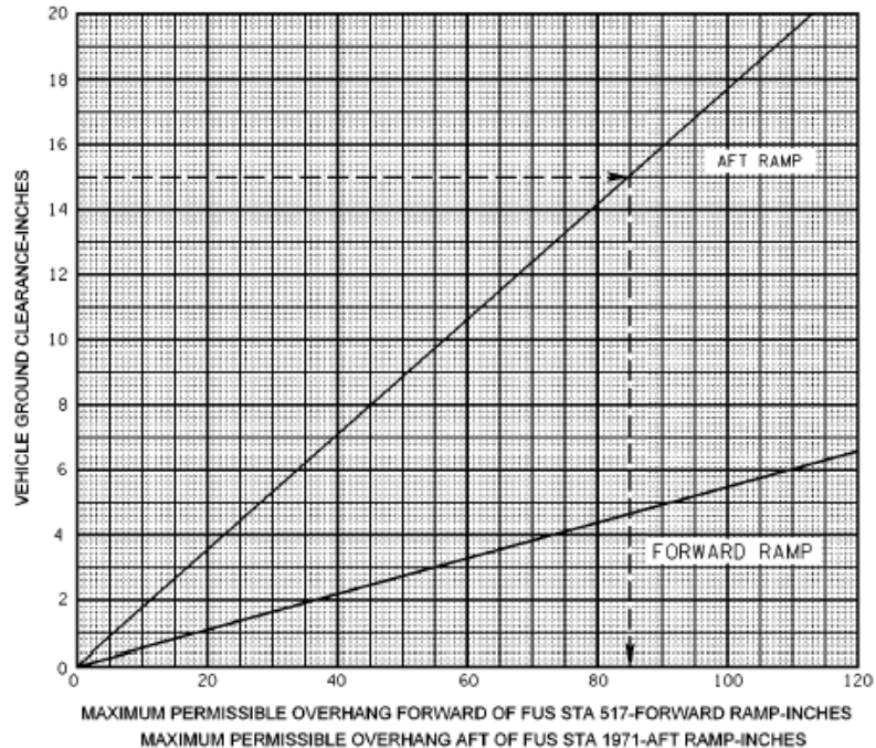
FIGURE B-28. Parking overhang limits.
