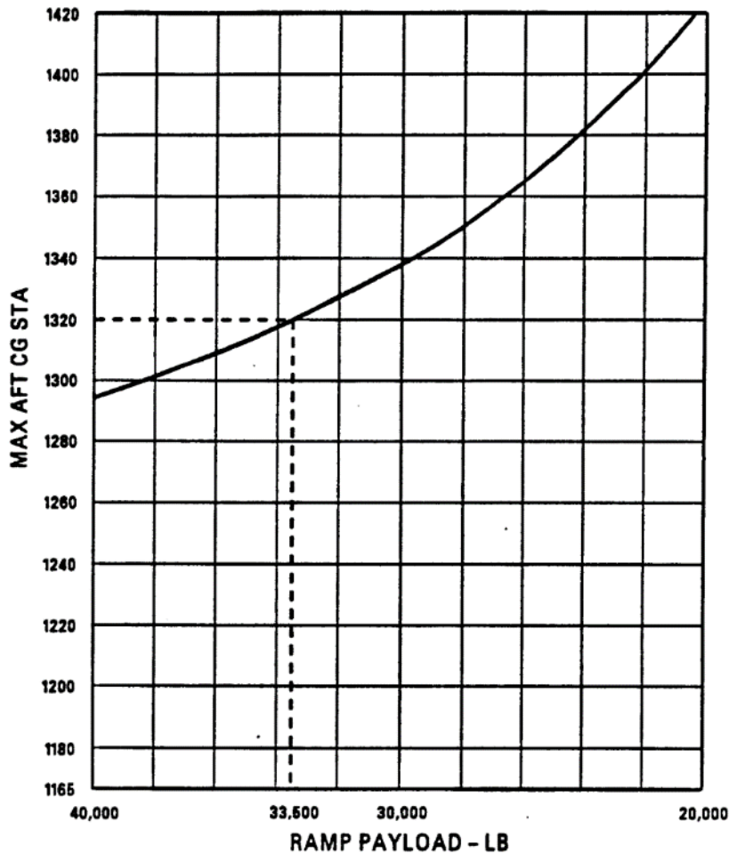
FIGURE B-70. Allowable in-flight ramp payload.
