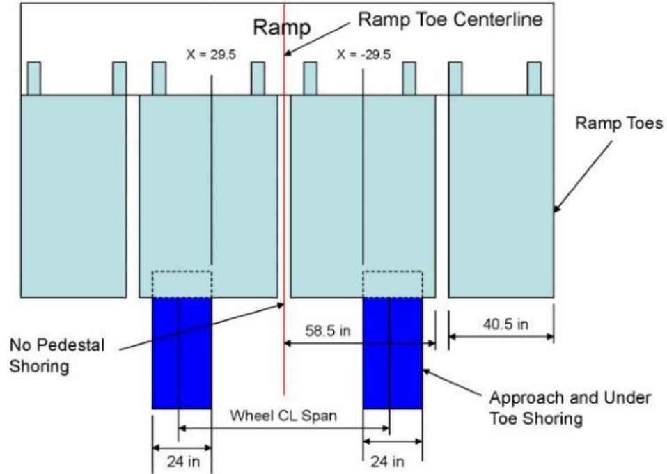
FIGURE B-59. C-17 minimum approach shoring width under ramp toes - (sheet 2 of 4).
