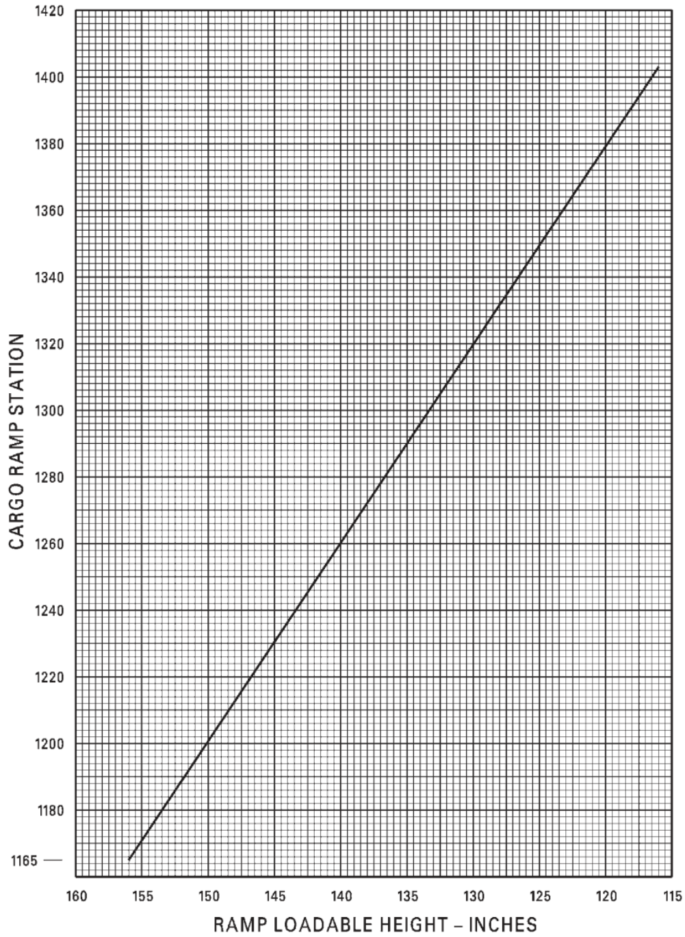
FIGURE B-58. Allowable in-flight ramp loadable height.
