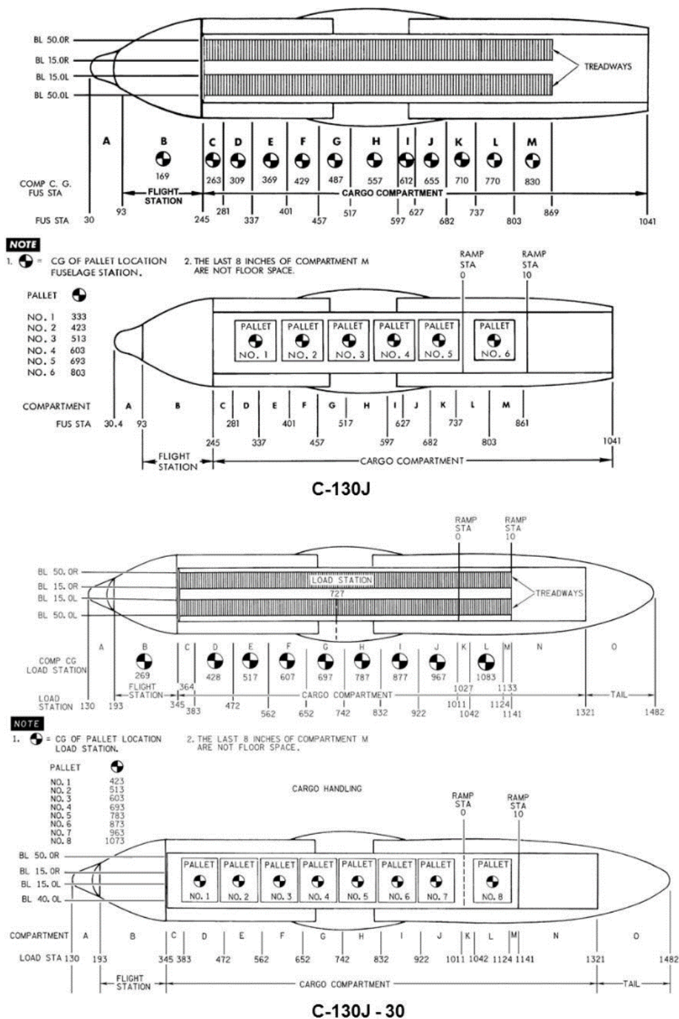
C-130J and -30
