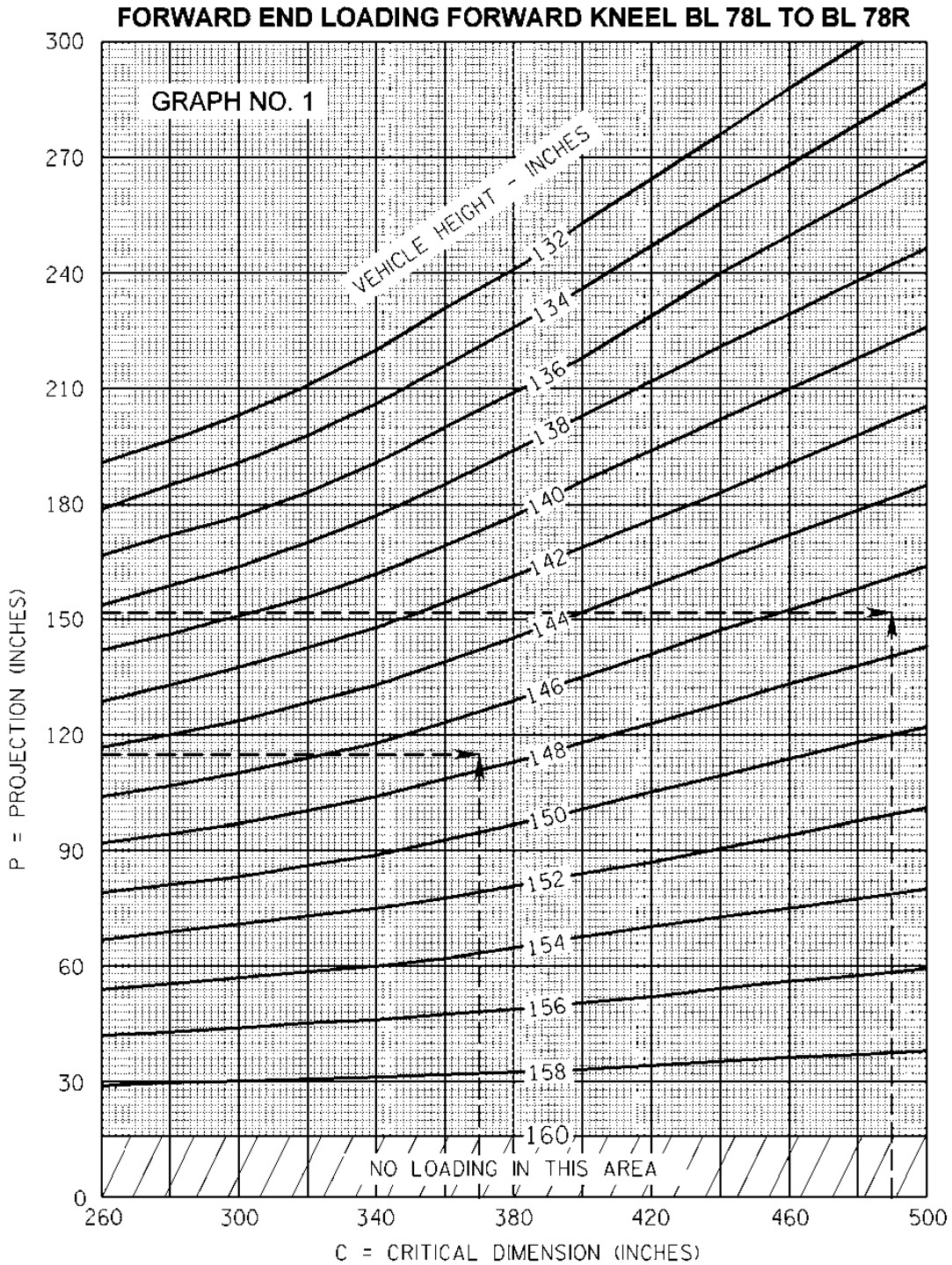
FIGURE B-10. Forward and aft end loading - vehicle projection limits.
