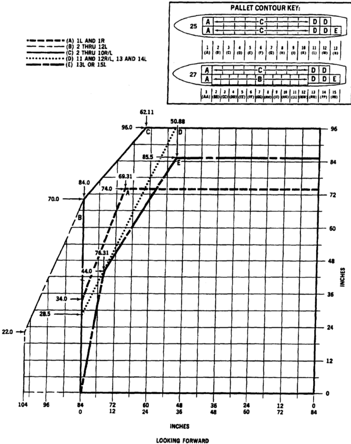
FIGURE B-106. Pallet contours and aisle configurations.
