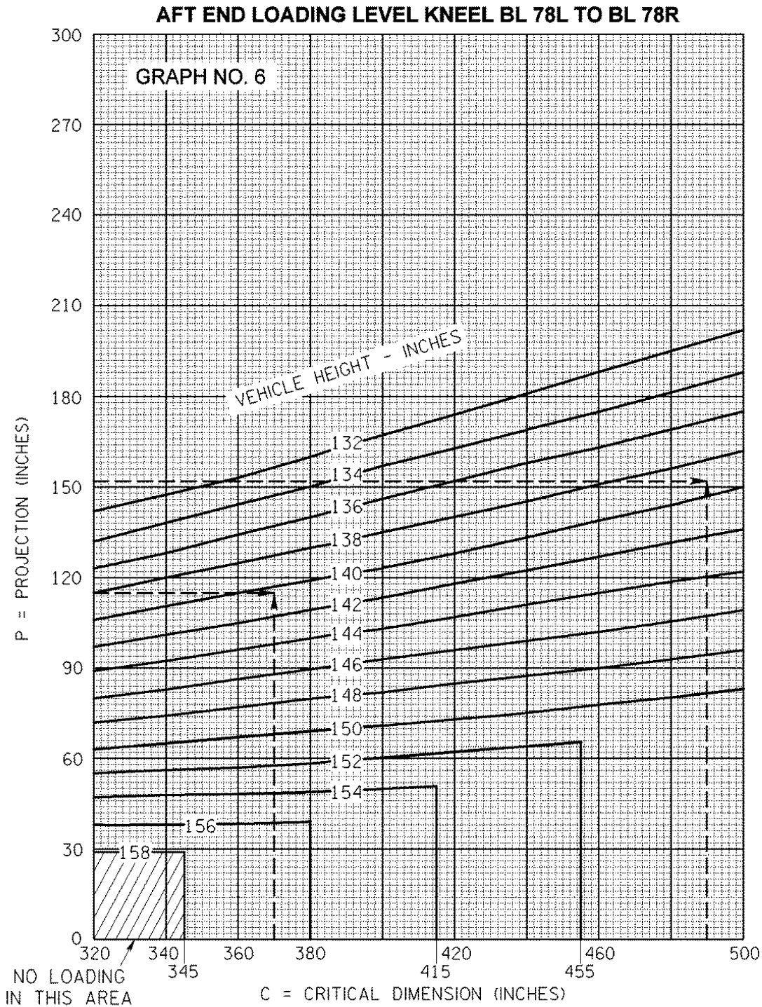
FIGURE B-15. Forward and aft end loading - vehicle projection limits.
