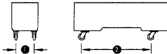
FIGURE B-133. Allowable load for hard rubber and steel wheels - Continued.
