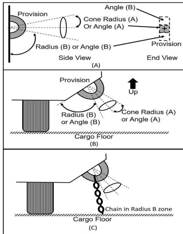
FIGURE A-33. Multiple chain restraint.
