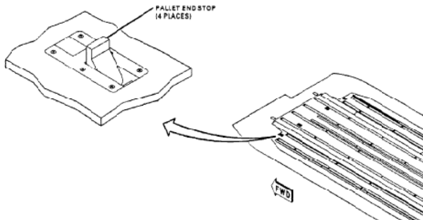
FIGURE B-68. C-17 logistic rail system.
