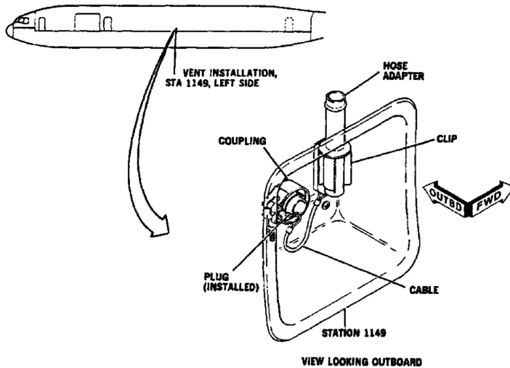
FIGURE B-122. Cargo compartment cryogenic vent.
