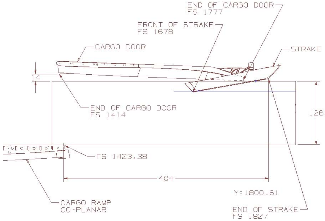
FIGURE B-51. C-17 straight-in loading envelope, side view.
