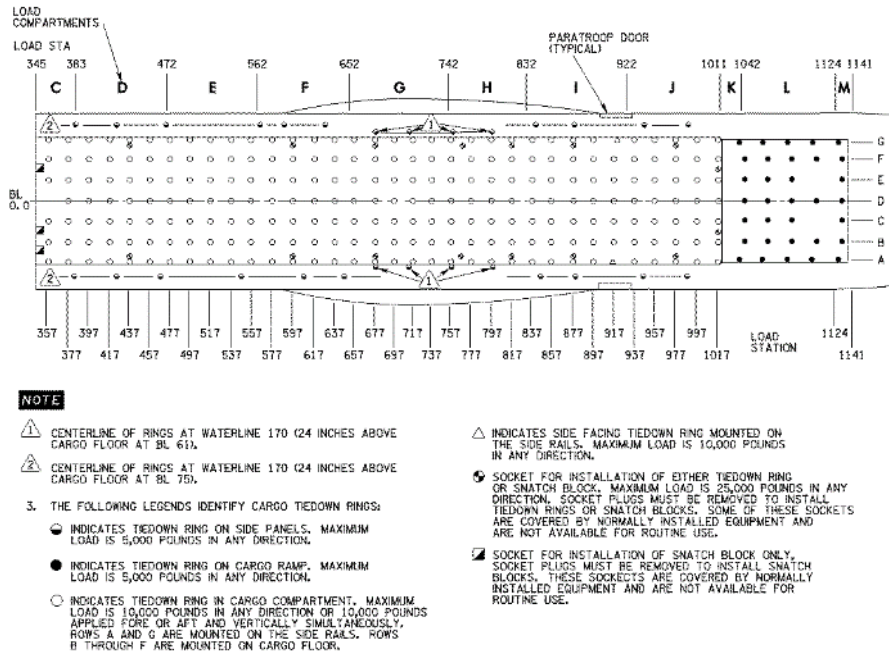
FIGURE B-100. C-130J-30 tiedown fittings locations.
