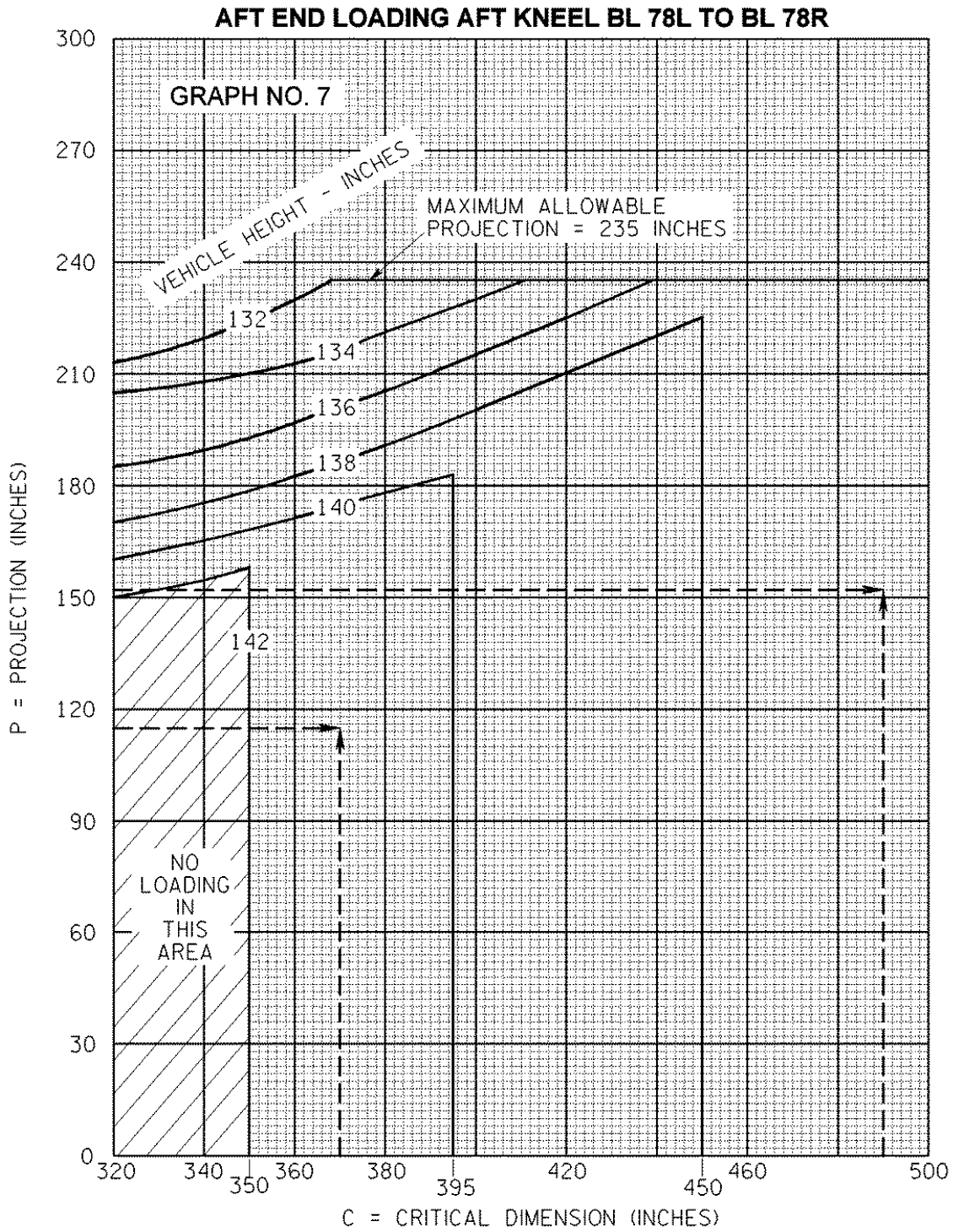
FIGURE B-16. Forward and aft end loading - vehicle projection limits.
