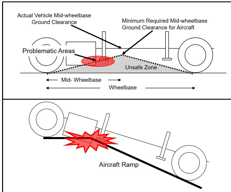
FIGURE A-2. Problematic areas for cresting.
