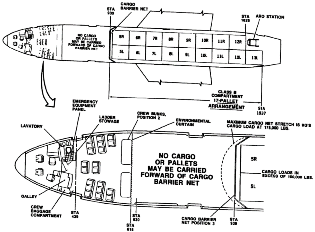
FIGURE B-111. Mixed cargo/personnel configuration.
