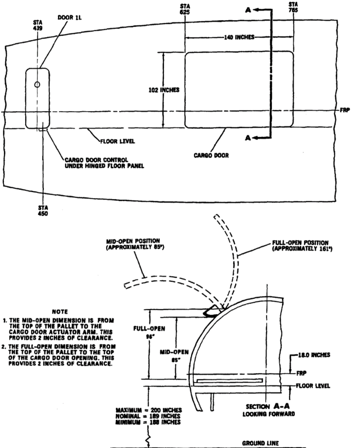
FIGURE B-112. Cargo door.
