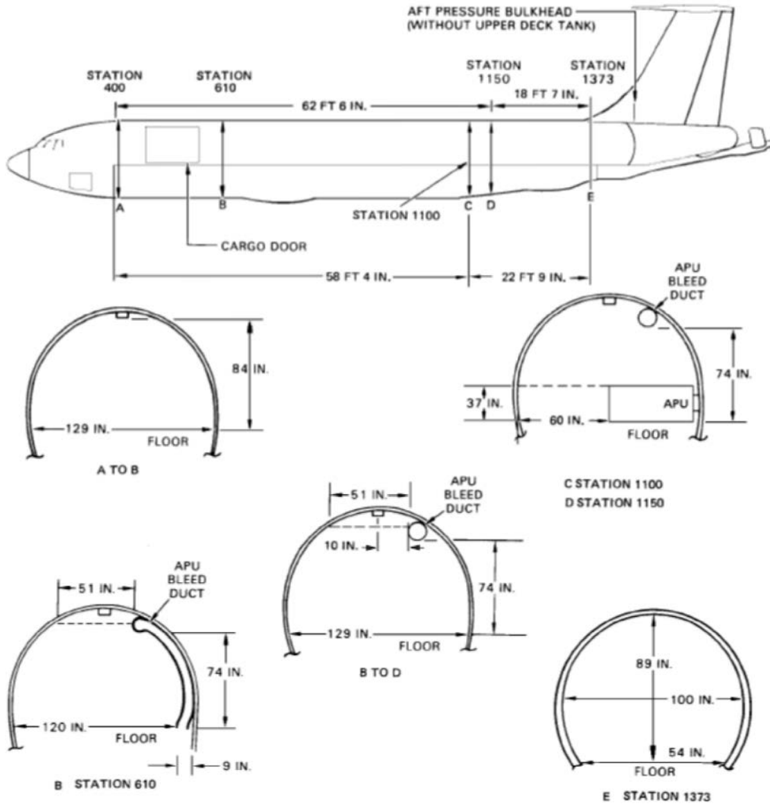
FIGURE B-127. KC-135 R/T cargo compartment.
