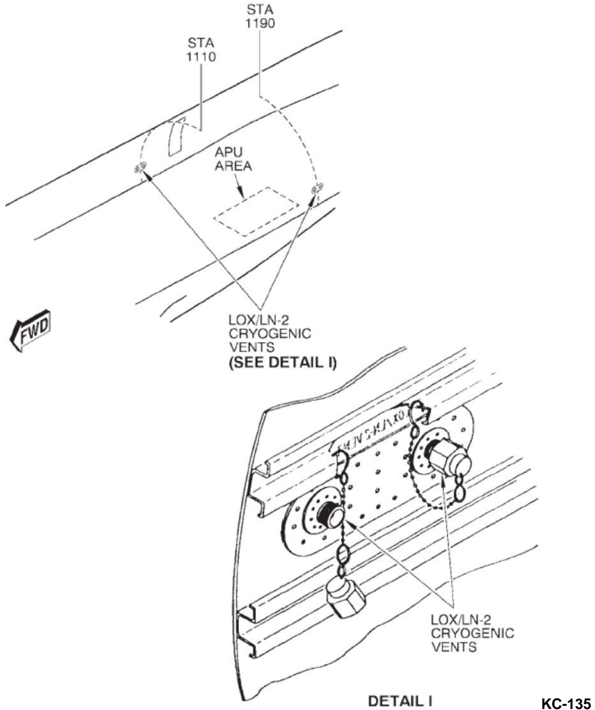
FIGURE B-137. KC-135 cryogenic vents.
