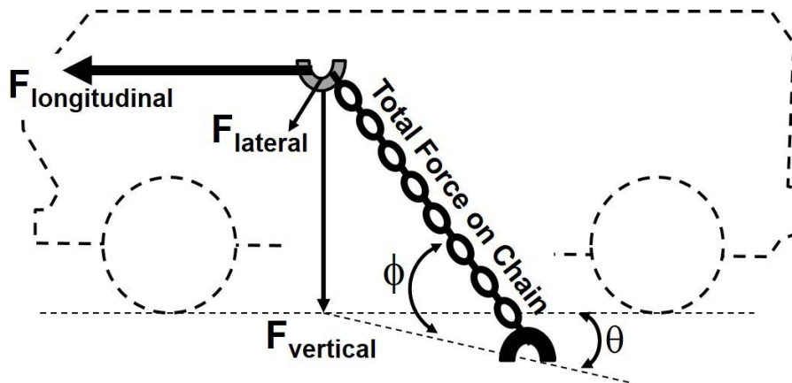
FIGURE A-35. Unsatisfactory bulk cargo restraint.
