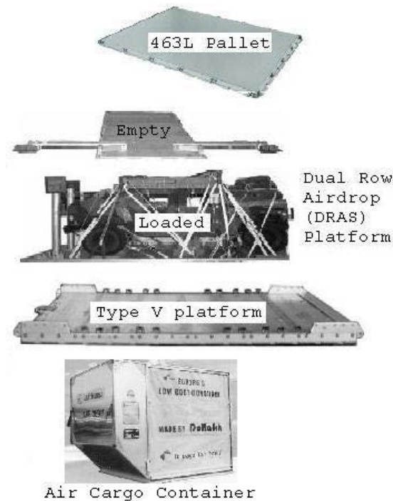
FIGURE A-17. Standard pallets and containers.
