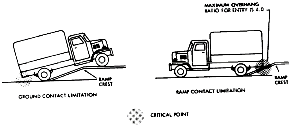
CHART B - PARKING OVERHANG LIMITS
