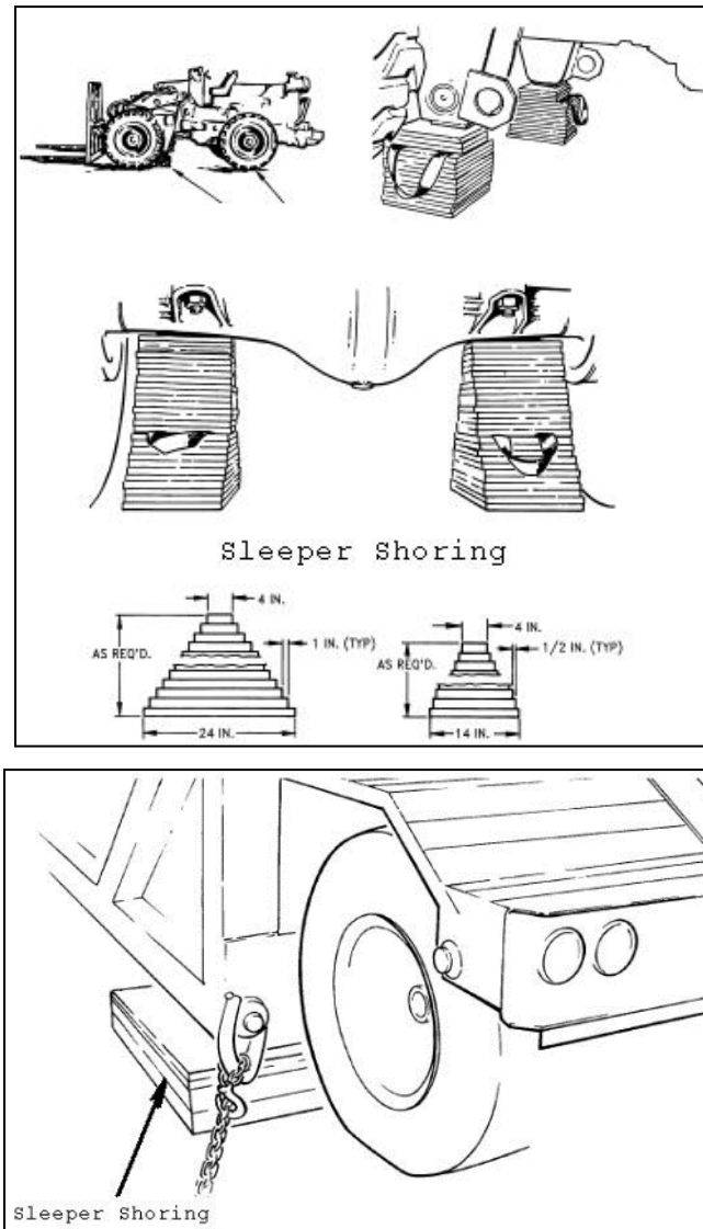
FIGURE A-45. Sleeper shoring.
