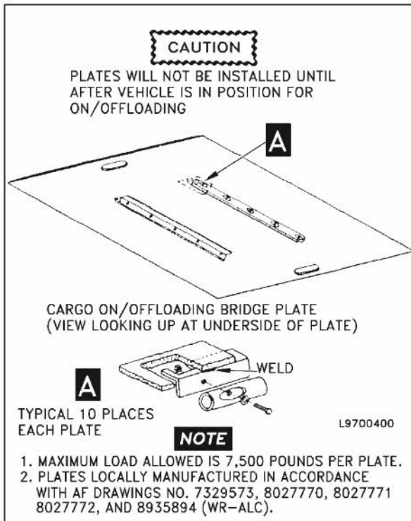
Bridge Plates
