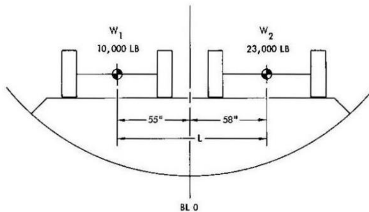
FIGURE B-33. Cargo maximum allowable lateral CG location (sheet 1 of 3).
