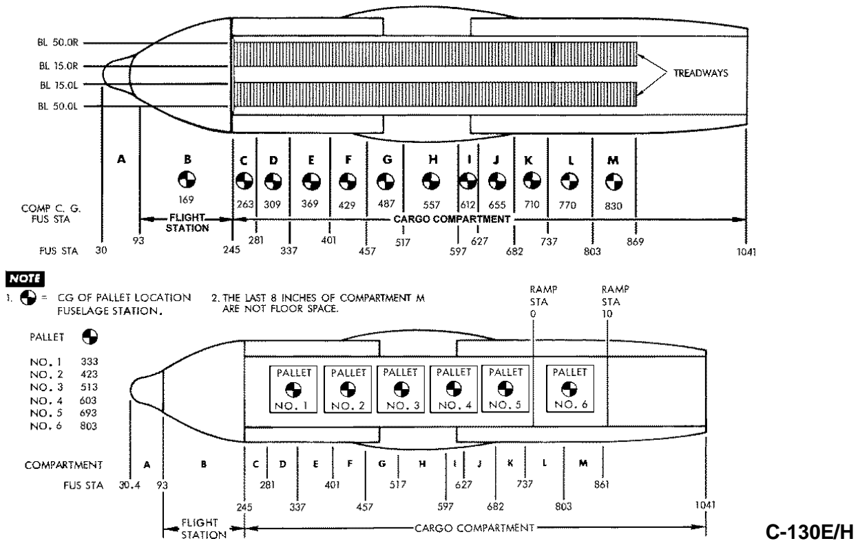
FIGURE B-89 C-130E/H compartments and pallet centroids.
