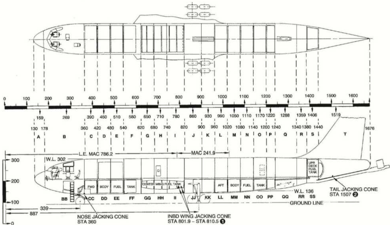
FIGURE B-126. Aircraft diagram (typical).
