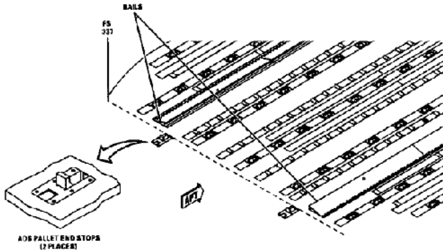
FIGURE B-67. C-17 ADS system (sheet 1 of 2).
