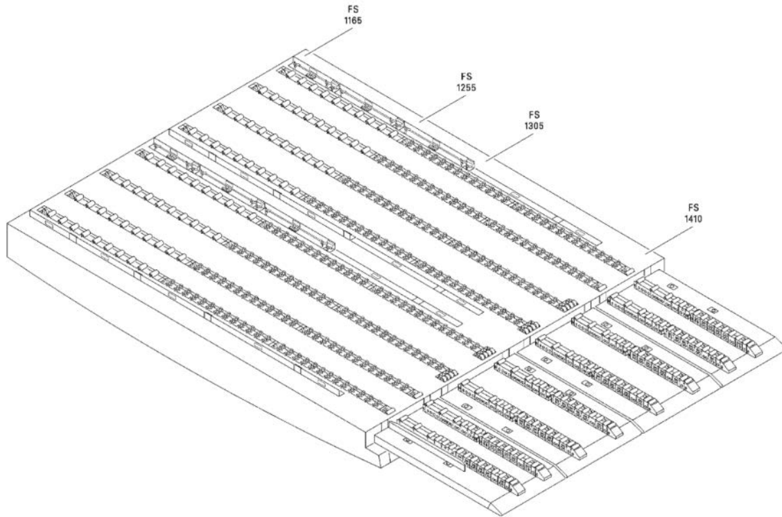
FIGURE B-73. C-17 ramp and ramp toes configured for dual row logistics system loading.
