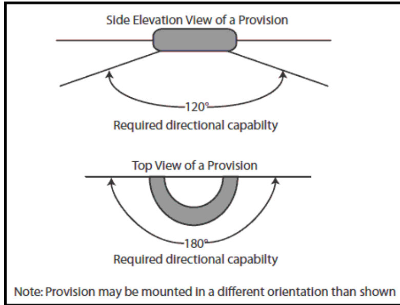
FIGURE 2. Tiedown rings.
