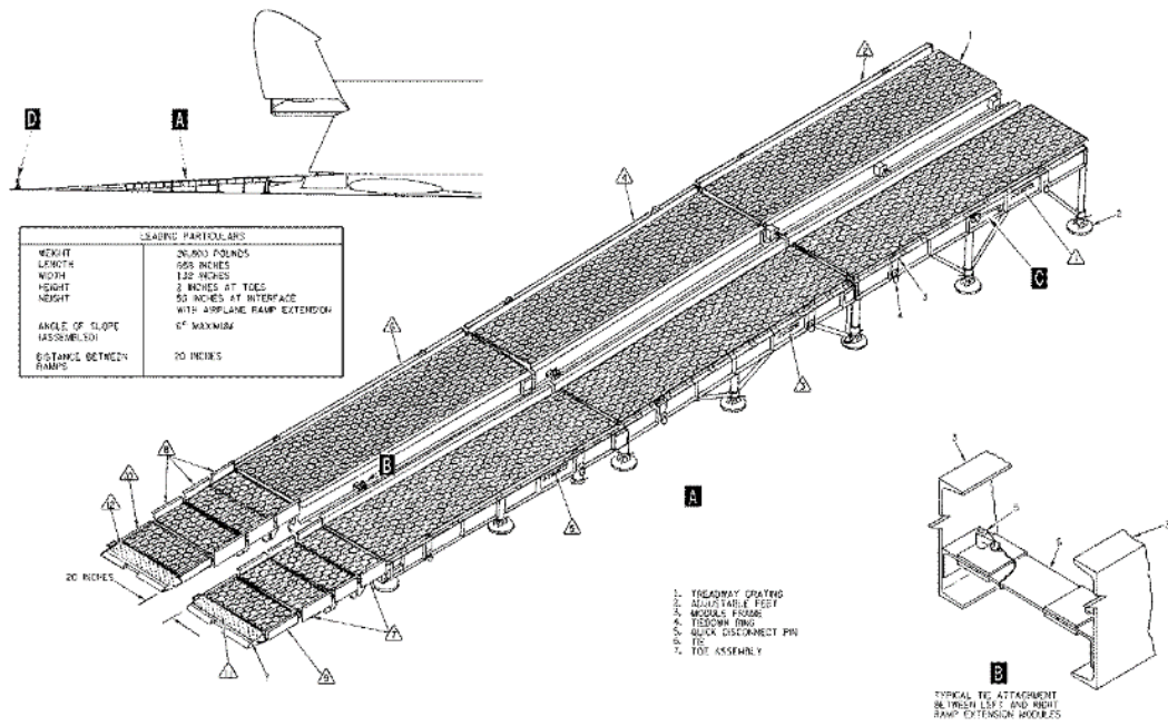
FIGURE B-30. Portable loading ramp extension.
