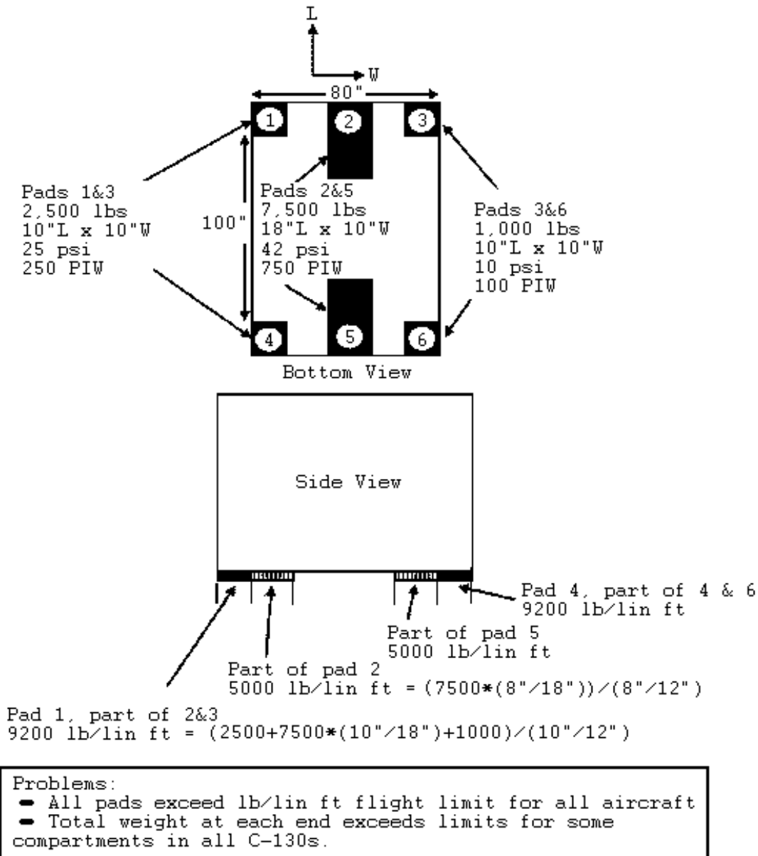
FIGURE A-20. Floor loading calculation.
