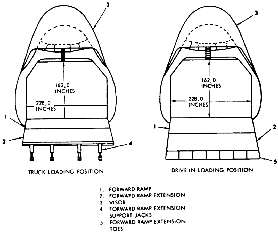
FIGURE B-3. Forward cargo opening dimension.
