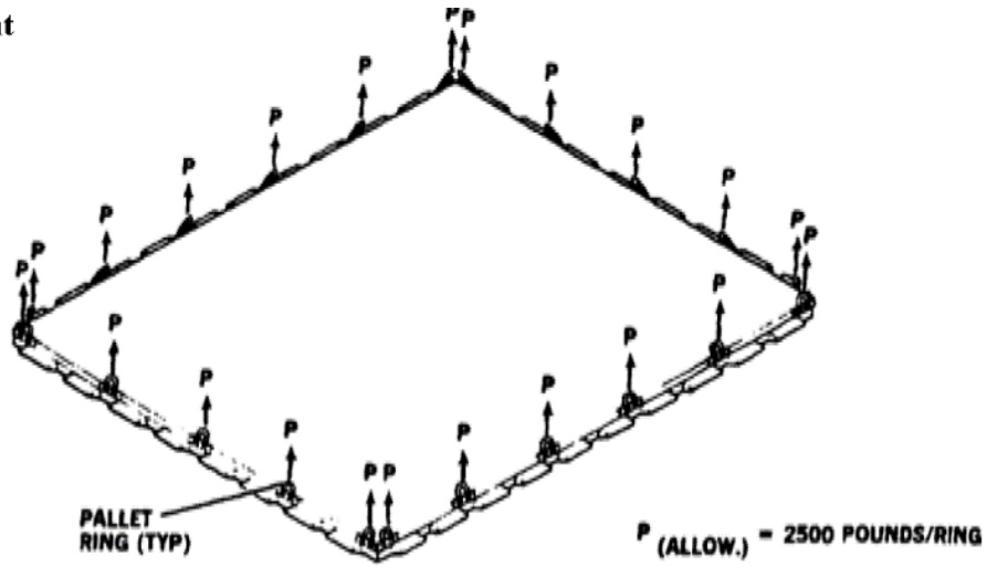
SINGLE HCU-6/E PALLETS
