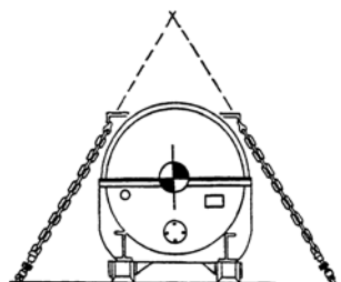
FIGURE A-30. CG location for effective restraint.
