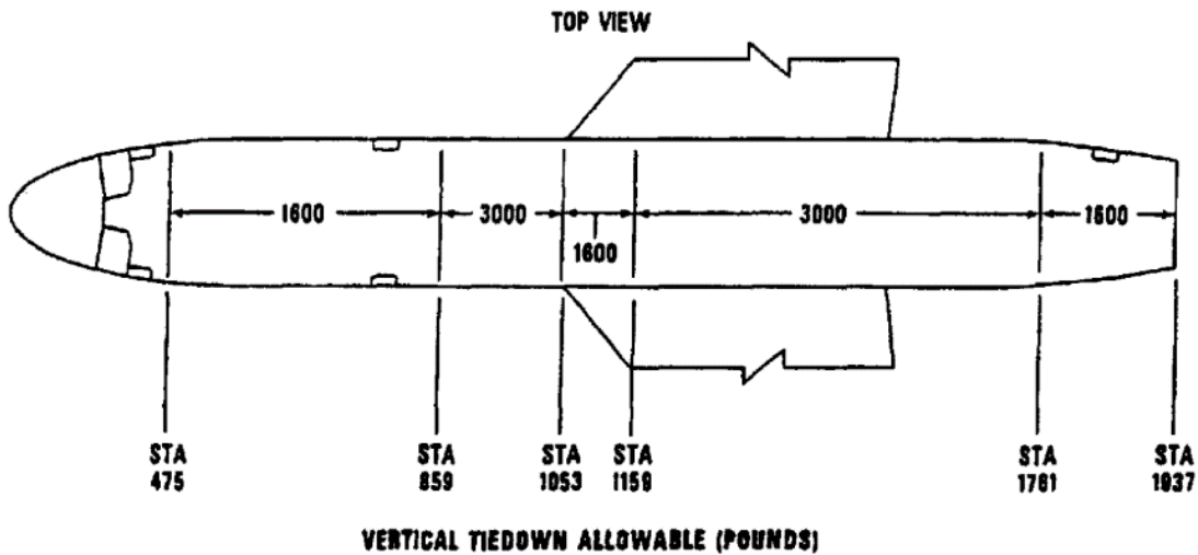
FIGURE B-120. A-7000 vertical tiedown allowables.
