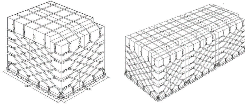
FIGURE A-6. Single and triple pallet loads.
