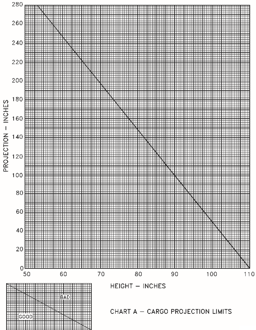
FIGURE B-84. Overhang and projection limits (cargo) - Continued.
