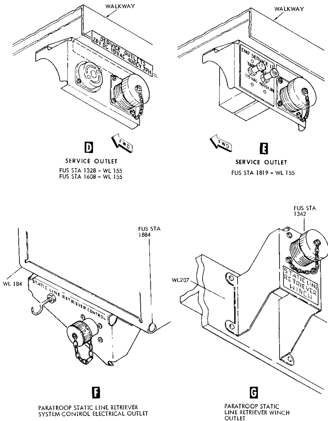
FIGURE B-46. Cargo compartment electrical outlets - Continued.
