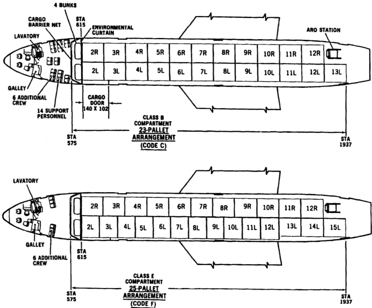
FIGURE B-107. Cargo compartment envelope.
