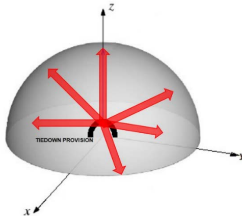
FIGURE A-32. Dimensions for tiedown analysis.
