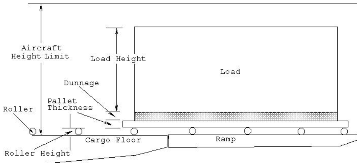
FIGURE A-14. Palletized cargo height.
