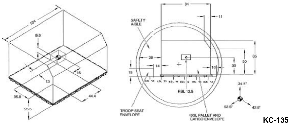
FIGURE B-129. Cargo contour.
