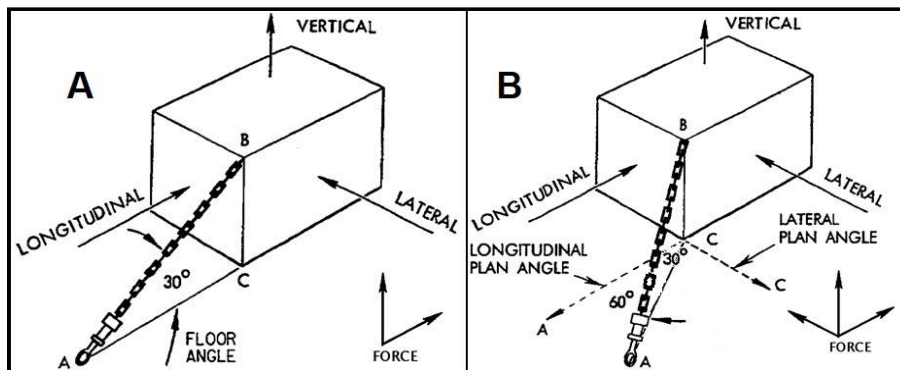
FIGURE A-28. Tiedown angles 2.
