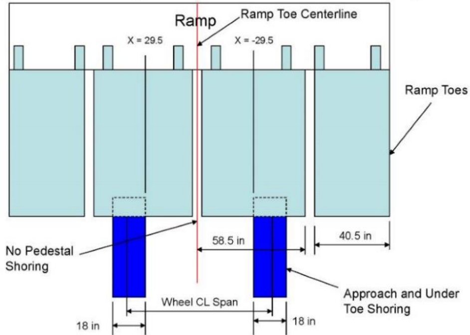
FIGURE B-59. C-17 minimum approach shoring width under ramp toes (sheet 1 of 4).
