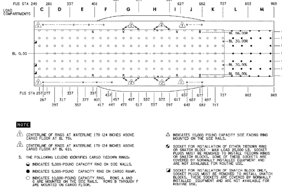
FIGURE B-99. C-130J tiedown fittings locations.
