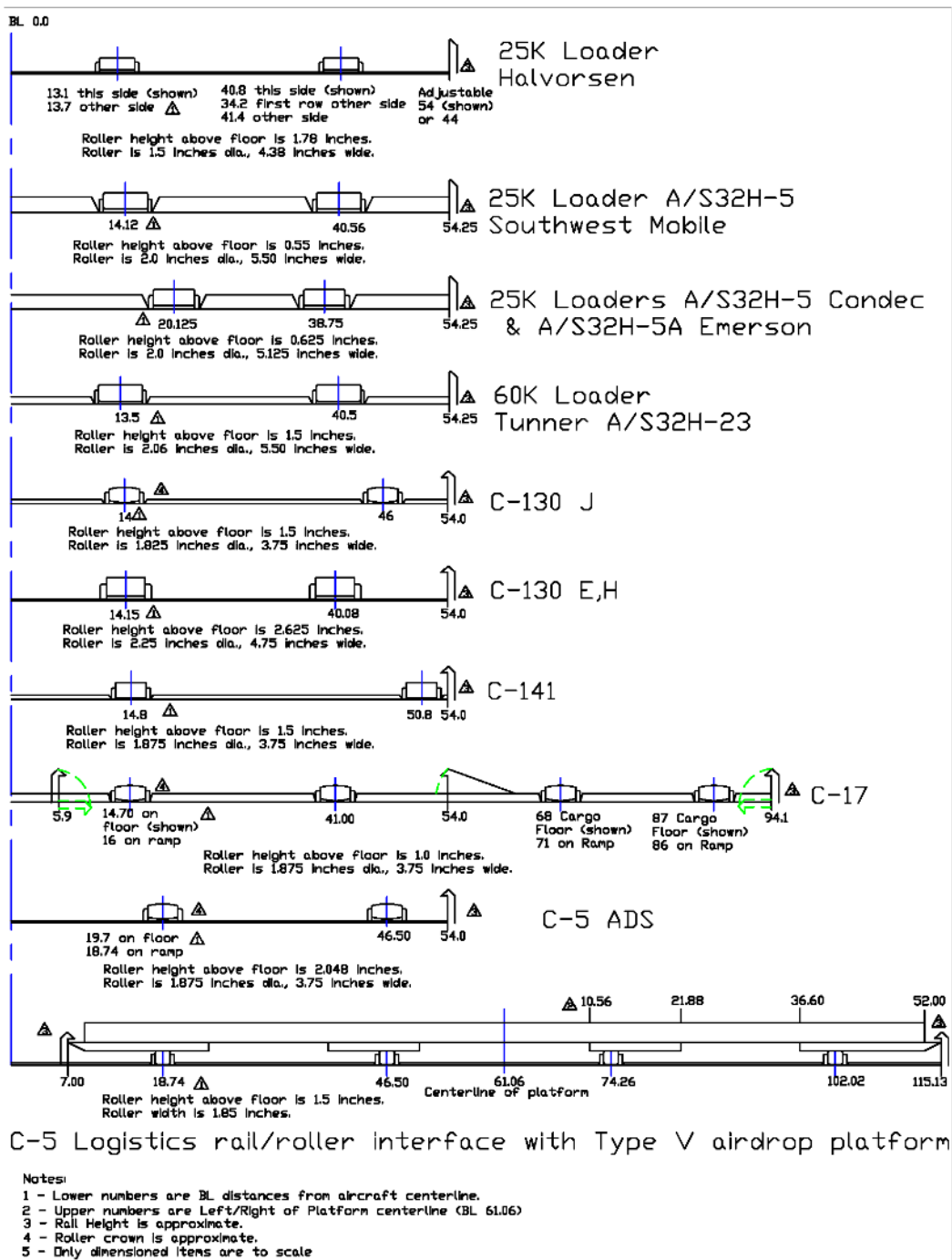
FIGURE A-11. Logistics rail/roller interface with type V airdrop platform.
