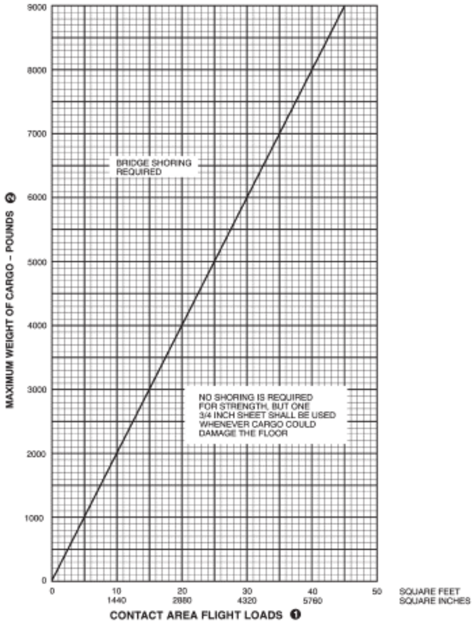
FIGURE B-131. Large area loads (greater than 1.5 square feet).
