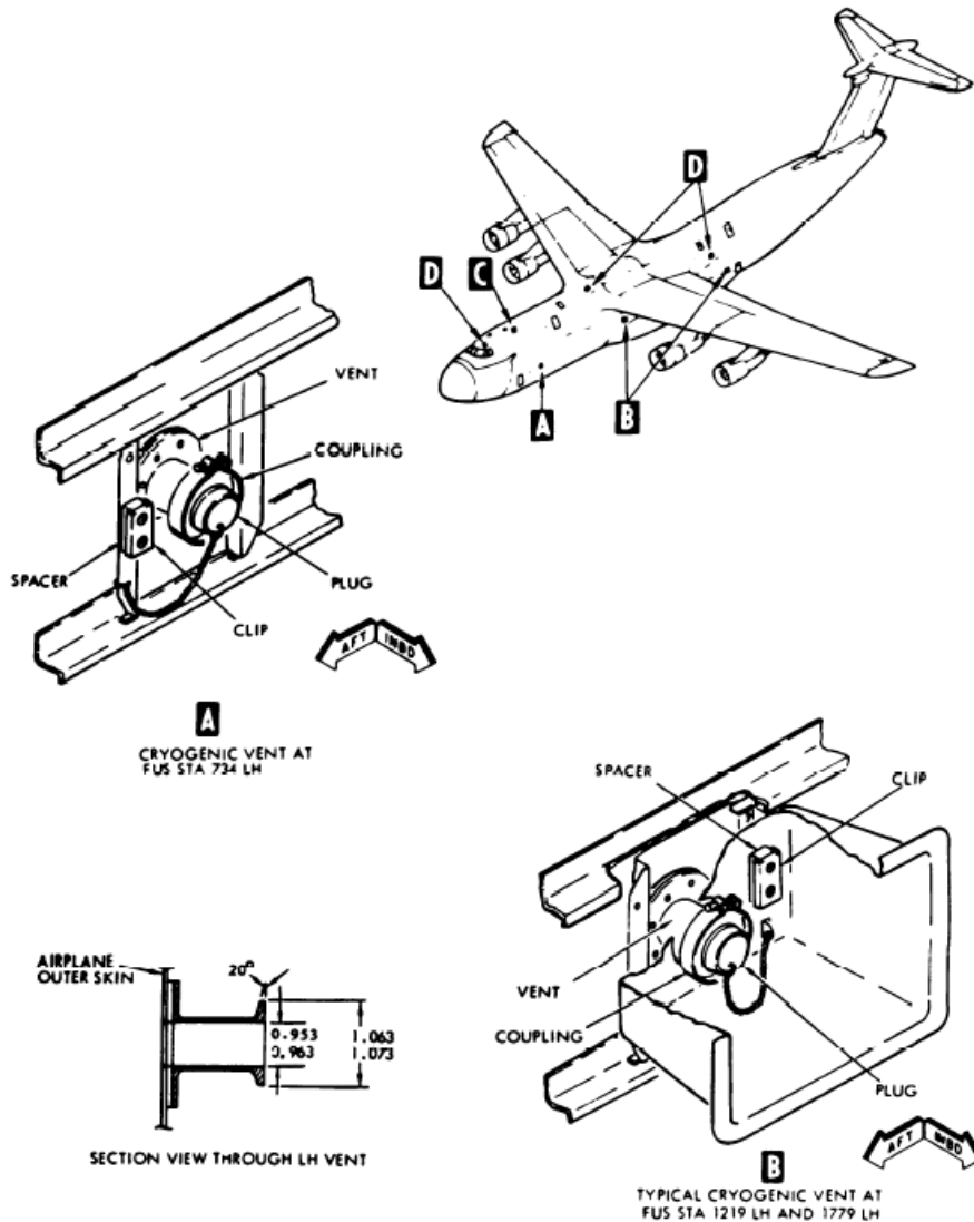
FIGURE B-45. C-5 overboard vents.
