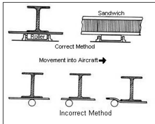
FIGURE 4. Pallet/roller interface.
