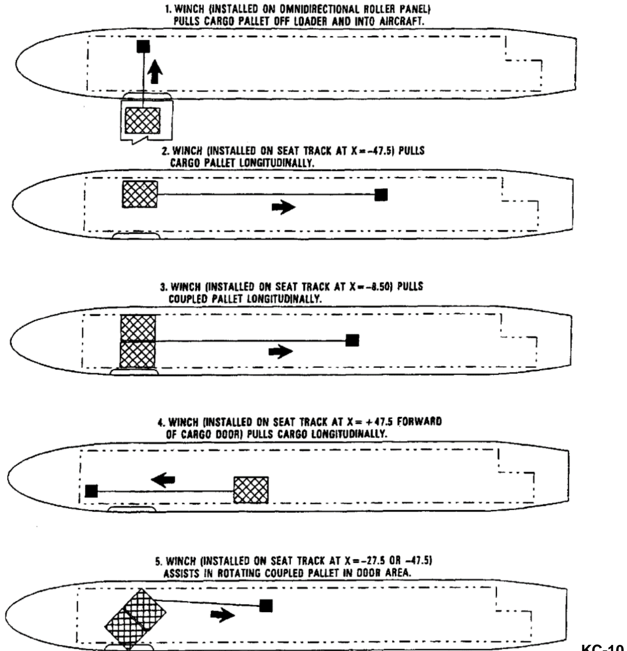
FIGURE B-124. Winching arrangements.
