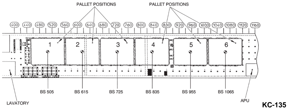
FIGURE B-128. Cargo roller handling system (six pallets installed).
