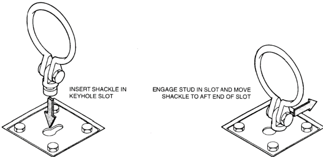
Figure Installation of Tiedown Shackles 5000 and 10,000 pound capacity
