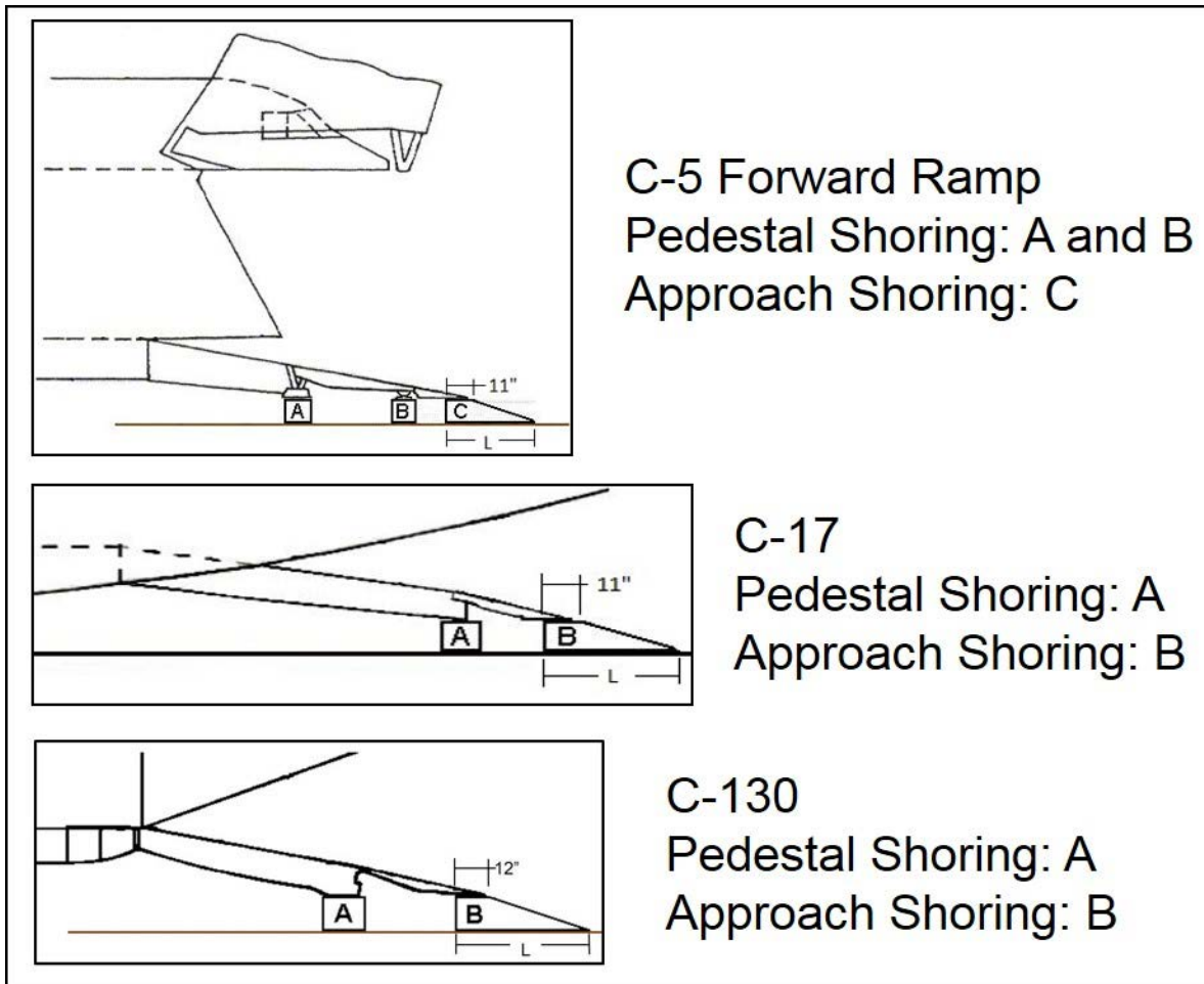
FIGURE A-40. Pedestal shoring.
