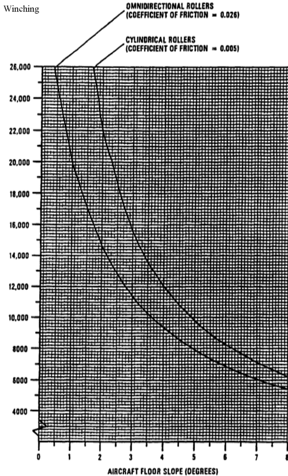
FIGURE B-125. Maximum capability of cargo winch on sloped aircraft floor.
