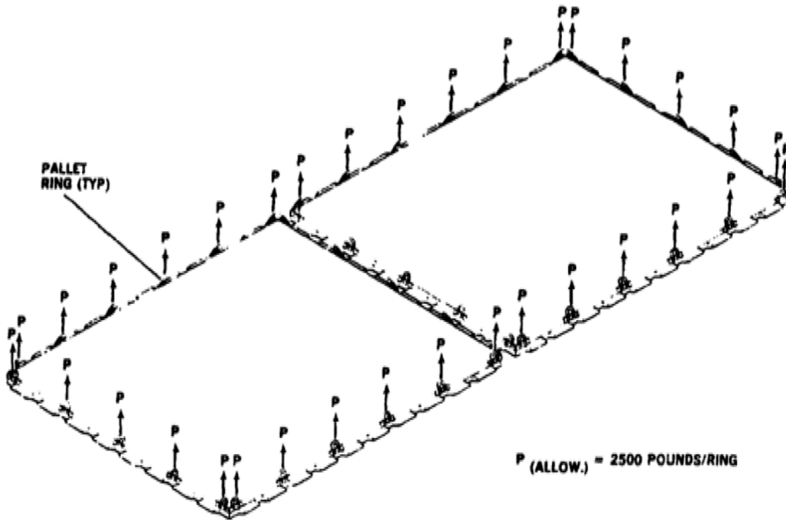
COUPLED HCU-6/E PALLETS
