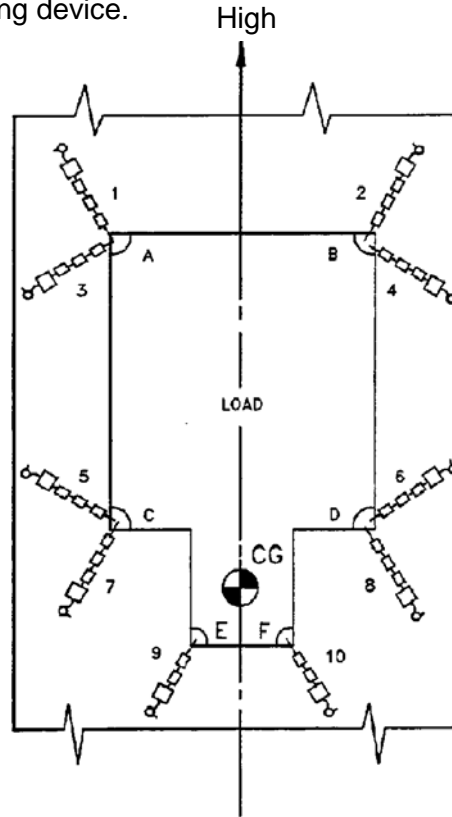
FIGURE A-31. Sample tiedown pattern.
