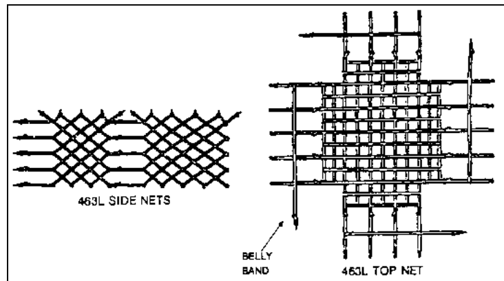
FIGURE A-7. Top and side netting.
